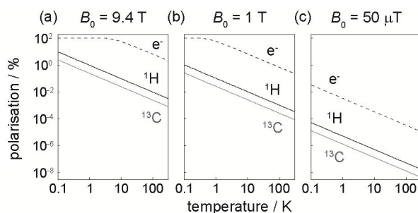
Figure 1. Polarisation level as a function temperature for 13 C nuclei (grey lines), 1 H nuclei (black lines) and unpaired electrons (dashed lines) with (a) B_0 = 9.4 T, (b) B_0 = 1 T, and (c) B_0 = 50 \mu T.
