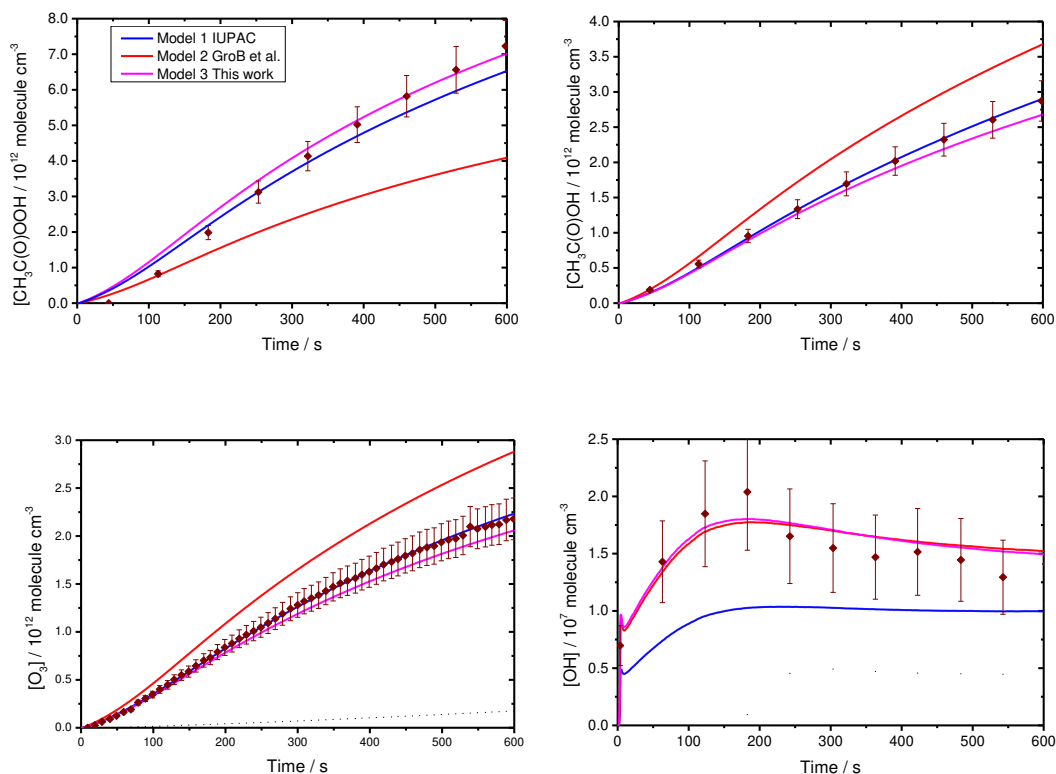
Figure 5. Comparison of the measured \text{CH}_3\text{C}(\text{O})\text{OOH} (a), \text{CH}_3\text{C}(\text{O})\text{OH} (b), \text{O}_3 (c), and OH (d) with various modelling scenarios, displayed as a function of time for experiment P2 conducted at 1000 mbar and 293 K. Error bars are representative of the uncertainty in the FTIR (for a–c) and FAGE (d) measurement techniques to \pm 2\sigma . Chemical simulations were conducted with different k_{(\text{R}5)} and branching ratios \alpha_{(\text{R}5\text{a})} : \alpha_{(\text{R}5\text{b})} : \alpha_{(\text{R}5\text{c})} . Model 1 (IUPAC): k_{(\text{R}5)} = 1.4 \times 10^{-11} \text{ cm}^3 \text{ molecule}^{-1} \text{ s}^{-1} , \alpha_{(\text{R}5\text{a})} : \alpha_{(\text{R}5\text{b})} : \alpha_{(\text{R}5\text{c})} = 0.44 : 0.15 : 0.41 . Model 2 (Groß et al., 2014b): k_{(\text{R}5)} = 2.1 \times 10^{-11} \text{ cm}^3 \text{ molecule}^{-1} \text{ s}^{-1} , \alpha_{(\text{R}5\text{a})} : \alpha_{(\text{R}5\text{b})} : \alpha_{(\text{R}5\text{c})} = 0.23 : 0.16 : 0.61 . Model 3 (This work): k_{(\text{R}5)} = 2.4 \times 10^{-11} \text{ cm}^3 \text{ molecule}^{-1} \text{ s}^{-1} , \alpha_{(\text{R}5\text{a})} : \alpha_{(\text{R}5\text{b})} : \alpha_{(\text{R}5\text{c})} = 0.35 : 0.10 : 0.55 .
