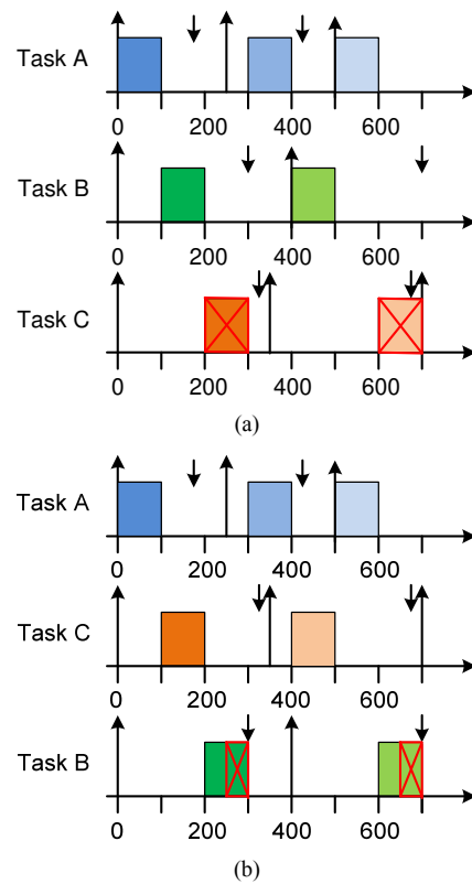
Figure 8: Deadline Monotonic priority ordering is not optimal for fixed priority non-pre-emptive scheduling.
