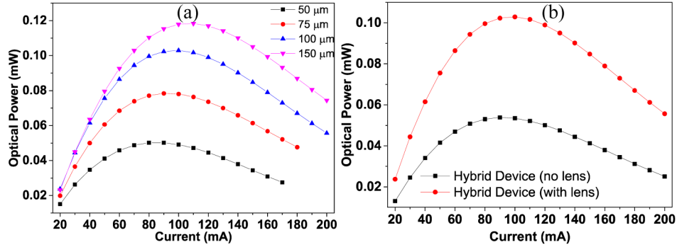
Fig. 3. a) L-I curve for the NM-hybrid devices and b) power enhancement by addition of the lens for the 100 \mu\text{m} device.
