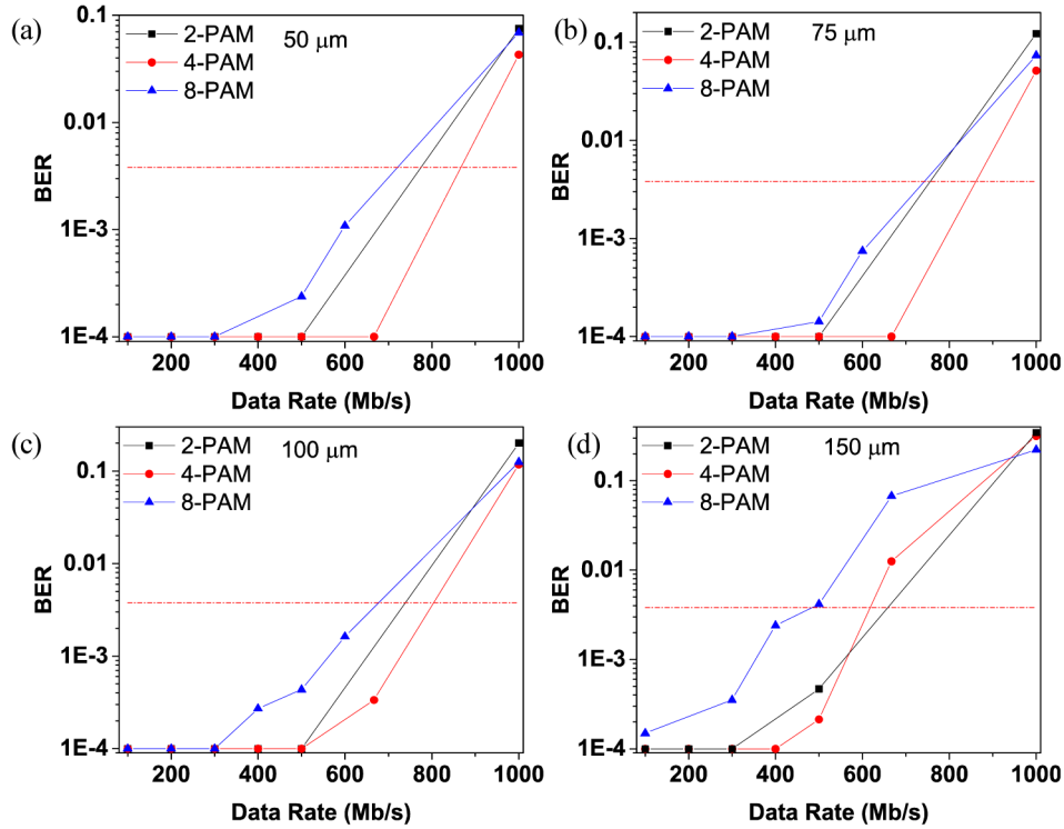
Fig. 7. BER vs Data Rate for the hybrid devices a) 50\mu\text{m} \times 50\mu\text{m} pixels, b) 75\mu\text{m} \times 75\mu\text{m} pixels, c) 100\mu\text{m} \times 100\mu\text{m} pixels and d) 150\mu\text{m} \times 150\mu\text{m} pixels.
