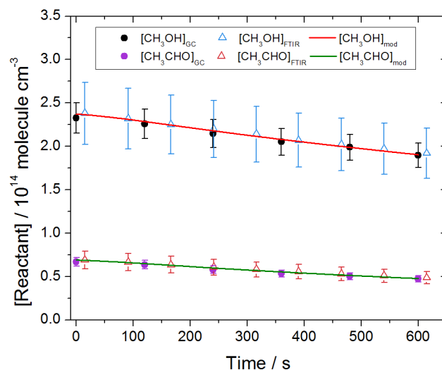
Figure 1. Decay of reactants \text{CH}_3\text{CHO} and \text{CH}_3\text{OH} from experiment P11 measured simultaneously using FTIR and GC-FID conducted at 1000 mbar and 298 K. Error bars are representative of the uncertainty in the calibration of the FTIR and GC-FID ( \pm 2\sigma ). Measurements are in excellent agreement within their respective uncertainties. Chemical simulation was conducted using the reaction scheme outlined in Table 2 using k_{(\text{R5})} = 2.35 \times 10^{-11} \text{ cm}^3 \text{ molecule}^{-1} \text{ s}^{-1} and \alpha_{(\text{R5a})} : \alpha_{(\text{R5b})} : \alpha_{(\text{R5c})} = 0.38 : 0.11 : 0.5 . Model concentrations for \text{CH}_3\text{CHO} and \text{CH}_3\text{OH} were observed to agree well with the experimental data, confirming accurate prediction of the reactant decays, and therefore the j(\text{Cl}_2) photolysis rate ( = (8 \pm 1) \times 10^{-5} \text{ s}^{-1} ).
