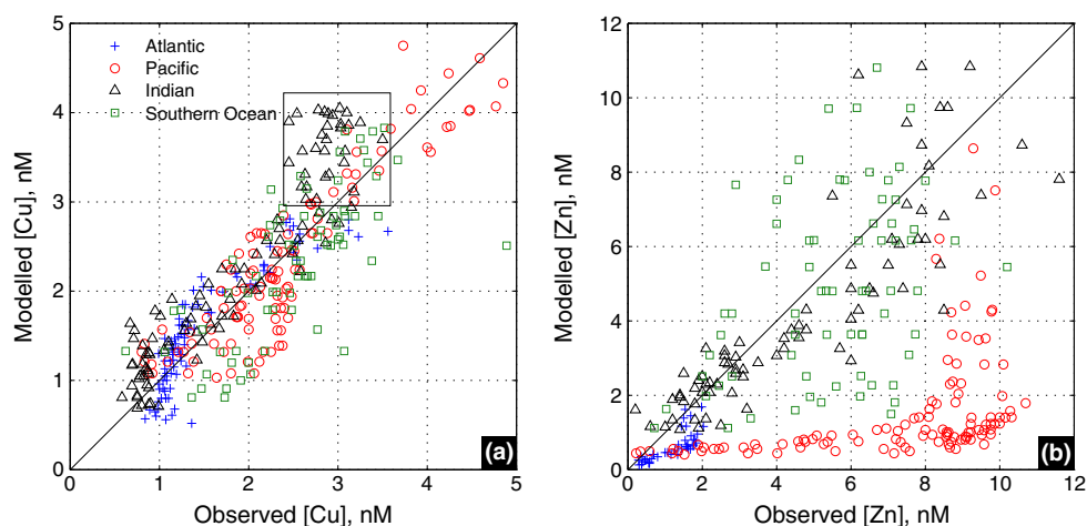
Figure 4. Fits of the reversible scavenging model to the global data sets of dissolved (a) Cu and (b) Zn. The solid line is the 1:1 relationship predicted for a perfect match of model to data. For Cu, the data and model match remarkably well, even at this global scale. Boxed Indian Ocean data are discussed in the text. For Zn, the fit is poor, especially in the Pacific.
