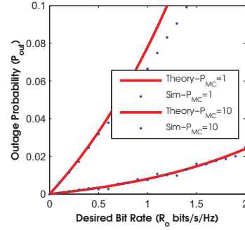
Figure 3. Outage probability of MU vs. desired bit rate R_o in bits/s/Hz for varying values of P_{MC} with \sigma^2 = -70 dB/Hz, \lambda_{LP} = 0.48 \times 10^{-3} , \rho_{LS} = 0.3 and \alpha = 4 (see Eq. (20)).
