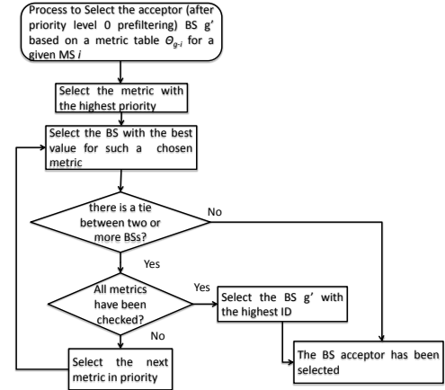
Figure 3. Flowchart of the sorting phase after pre-filtering in HHEA-DBC.
