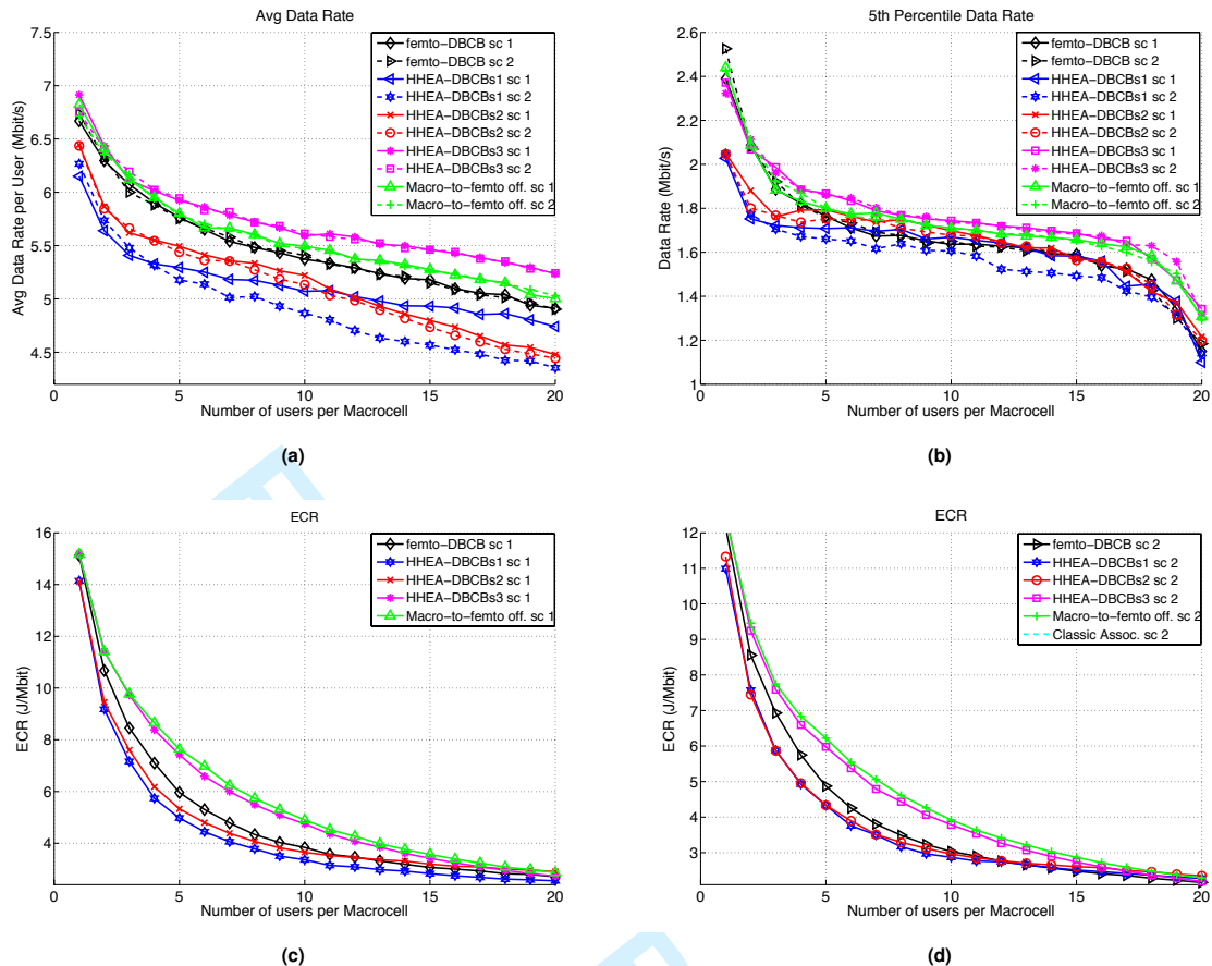
Figure 8. a) Average Data Rate per User b) 5th percentile of Data Rate per user c) Energy Consumption Rating (ECR) [J/Mbit] for scenario 1 and d) ECR for scenario 2, for each one of the algorithms analyzed
