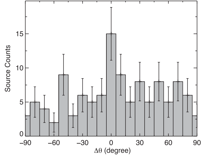
Figure 3. Difference between the clump position angles and the Galactic mid-plane. The bin size is 10° and the errors are estimated using Poisson statistics.
