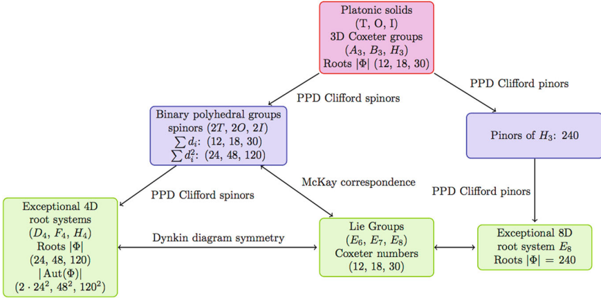
FIGURE 3. Web of connections putting the original trinitities and McKay correspondence into a much wider context. The connection between the sum of the dimensions of the irreducible representations d_i of the binary polyhedral groups and the Coxeter number of the Lie algebras actually goes all the way back to the number of roots in the 3D root systems (12, 18, 30). These then induce the binary polyhedral groups (linked via the McKay correspondence to the E -type affine Lie algebras) and the 4D root systems via the Clifford spinor construction. The new pinor construction links H_3 directly with E_8 explaining the latter entirely within 3D geometry
