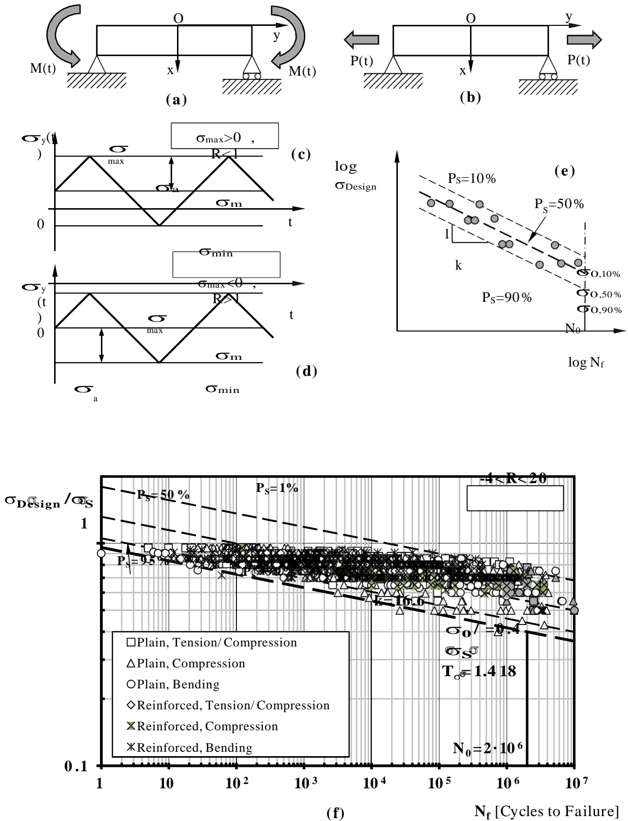
Figure 1. Concrete beam loaded in cyclic bending (a) and subjected to cyclic axial loading (b); load histories characterised by different values of the load ratio (c, d); Wöhler diagram and fatigue curves for different values of P_s (e); unifying Wöhler diagram to perform the fatigue assessment of un-notched plain and short fibre/particle reinforced concretes (grey markers = run outs) [1] (f).
