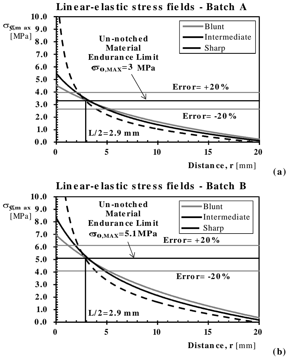
Figure 7. Local linear-elastic stress fields in the endurance limit condition and accuracy of the PM in estimating the high-cycle fatigue strength of the tested notched concrete.
