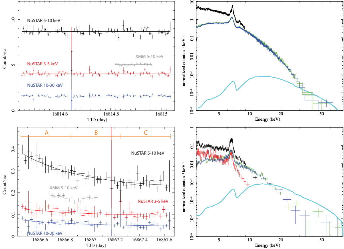
Fig. 3.— Light curves ( left ) and spectra ( right ) of the first ( top ) and second ( bottom ) observations. Left : XMM-Newton /EPIC-pn (grey, 5–10 keV) and NuSTAR /FPMA+FPMB (red: 3–5 keV, black: 5–10 keV, blue: 10–30 keV) light curves. Each light curve bin has 500 sec for the first observation and 2000 sec for the second observation, respectively. Right : XMM-Newton /EPIC-pn, MOS1 (black, red) and NuSTAR /FPMA, /FPMB (green, blue) spectra of \eta Car. The solid lines on the June 6 spectra show the best-fit model in Table 2. The solid cyan line on each panel for spectra shows the power-law component measured from the Suzaku observations (Hamaguchi et al. 2014b), convolved with the NuSTAR /FPMA response. We do not simultaneously fit the XMM-Newton and NuSTAR spectra for July 28 because the NuSTAR spectrum changed significantly during the second observation.
