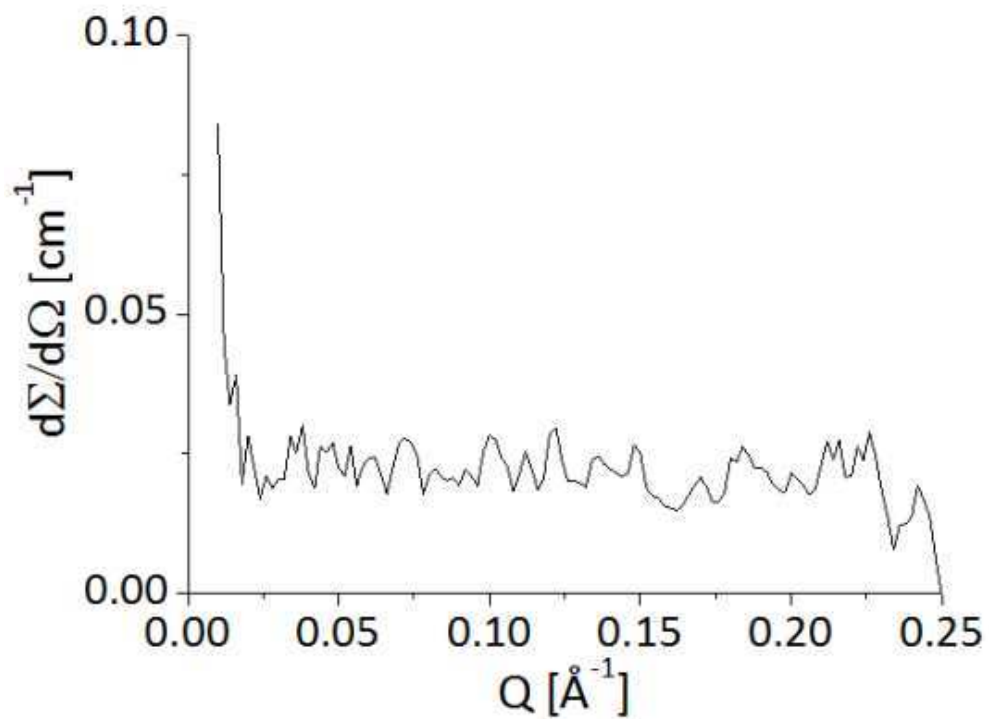
Figure 12: The differential scattering cross section from the instrument LOQ for the glutamine water solution at 298 K.
