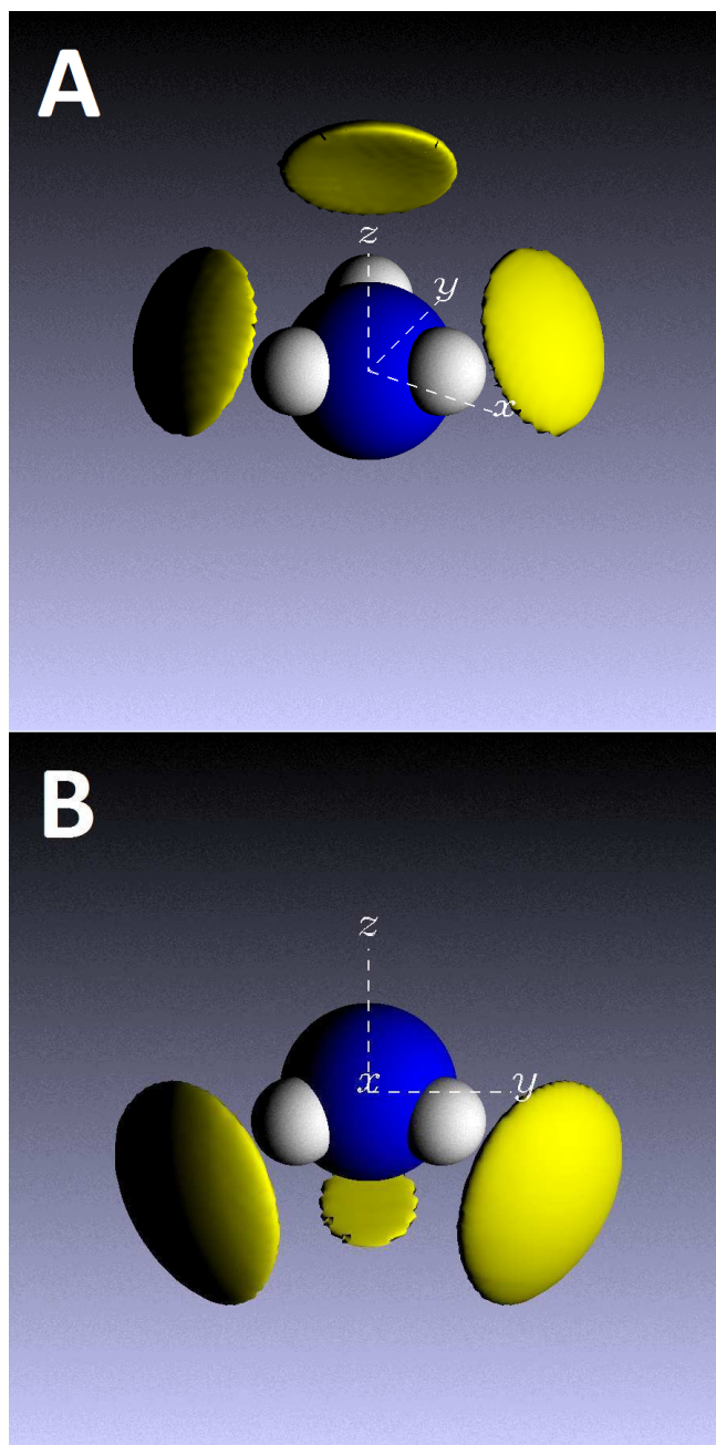
Figure 8: Spatial density function (SDFs) showing the distribution of water molecules around glutamine taken from the EPSR analysis of neutron diffraction data of aqueous glutamine surrounding (A) the backbone amine group of glutamine at a distance range of 2 – 3.42 Å (B) the side chain amine group of glutamine at a distance range of 2 – 3.45 Å. The distance ranges correspond to the first coordination shell of the corresponding N-Ow radial distribution function (Figure SI 2). The SDFs show 25% of the water molecules enclosed in this region.
