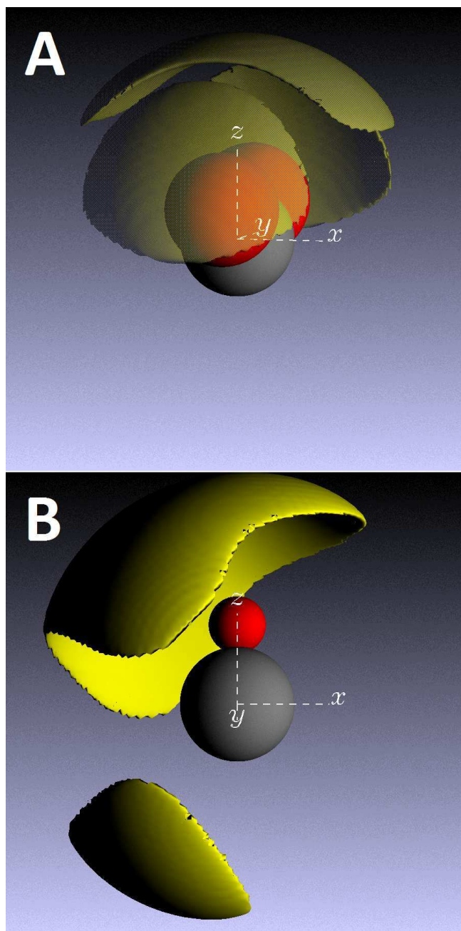
Figure 5: Spatial density function (SDFs) showing the distribution of water molecules around glutamine taken from the EPSR analysis of neutron diffraction data of aqueous glutamine. The yellow shaded areas represent the regions where there is a probability of finding a water molecule surrounding (A) the backbone carbonyl group of glutamine at a distance range of 2 – 4.28 Å and (B) the side chain carbonyl group of glutamine at a distance range of 2 – 4.41 Å. The distance ranges correspond to the first coordination shell of the corresponding C-Ow radial distribution function (Figure SI 1). The SDFs show 25% of the water molecules enclosed in this region.
