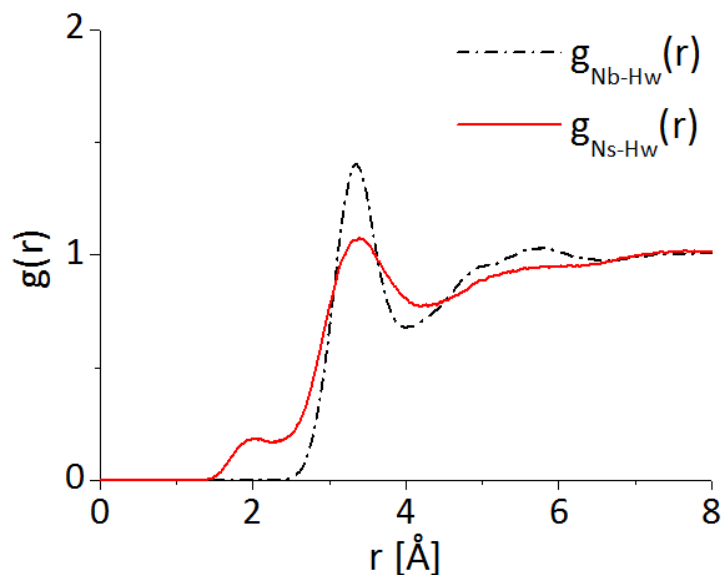
Figure 7. Glutamine – water interactions: Amine-water site-site partial radial distribution functions (RDFs) from the EPSR analysis of neutron diffraction data of the glutamine– water mixture. The g_{Nb-Hw} (dashed, black line) shows the ability of nitrogen atoms on the backbone (Nb) to coordinate water molecules ( H_W ). The g_{Ns-Hw} (solid, red line) shows the ability of nitrogen atoms on the side chain (Ns) to coordinate water molecules ( H_W ).
