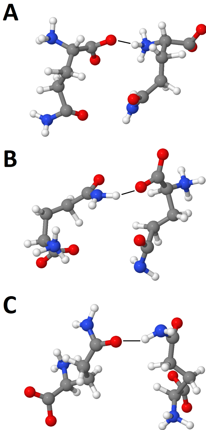
Figure 11: Representative snapshots from the EPSR simulation showing glutamine dimers which have formed from hydrogen bond interactions between (A) the backbone of one glutamine molecule and the backbone of another glutamine molecule (B) the backbone of one glutamine molecule and the side-chain of another glutamine molecule and (C) the side-chain of one glutamine molecule and the side-chain of another glutamine molecule
