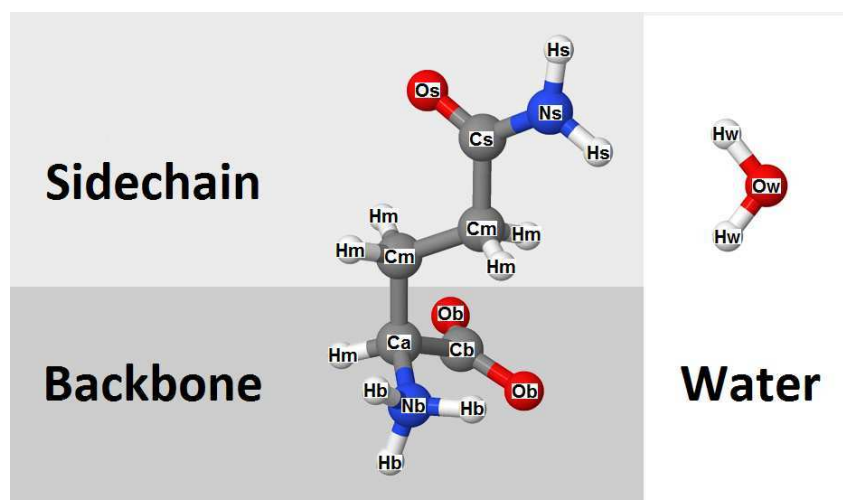
Figure 1. Representation of the glutamine and water molecules. The single atoms have been labelled according to the symbols used in the simulation and throughout this paper. For glutamine the carbon atoms are labelled Ca, Cb and Cm, the carbonyl oxygen atoms Ob and Os, the amine hydrogen atoms Hb and Hs, and the methyl hydrogen atoms Hm. The atoms Cb, Ob and Hb are in the glutamine backbone while the atoms Cs, Os and Hs are in the side chain. For water the oxygen atom is labelled OW and the water hydrogen atom HW.
