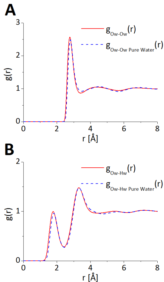
Figure 3. Water – water interactions: Water-water site-site partial radial distribution functions (RDFs) in a dilute aqueous glutamine solution. These include (A) g_{Ow-Ow} and (B) g_{Ow-Hw} . The RDFs are taken from the EPSR analysis of neutron diffraction data of the glutamine– water mixture (solid lines) and are compared with the same functions for pure water (dashed lines), where previously published neutron diffraction data 50 has been used to complete an EPSR simulation.
