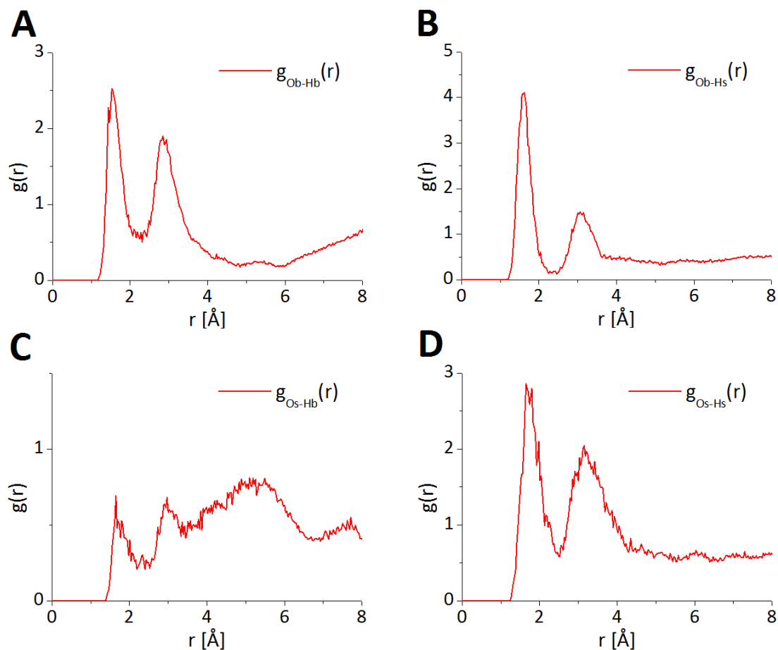
Figure 9: Glutamine – glutamine interactions: Glutamine-glutamine site-site partial radial distribution functions (RDFs) from the EPSR analysis of neutron diffraction data of the glutamine–water mixture. (A) The g_{Ob-Hb} shows the ability of oxygen atoms on the backbone (Ob) to coordinate hydrogen atoms on the backbone (Hb). (B) The g_{Ob-Hs} shows the ability of oxygen atoms on the backbone (Ob) to coordinate hydrogen atoms on the side chain (Hs). (C) The g_{Os-Hb} shows the ability of oxygen atoms on the side chain (Os) to coordinate hydrogen atoms on the backbone (Hb). (D) The g_{Os-Hs} shows the ability of oxygen atoms on the side chain (Os) to coordinate hydrogen atoms on the side chain (Hs).
