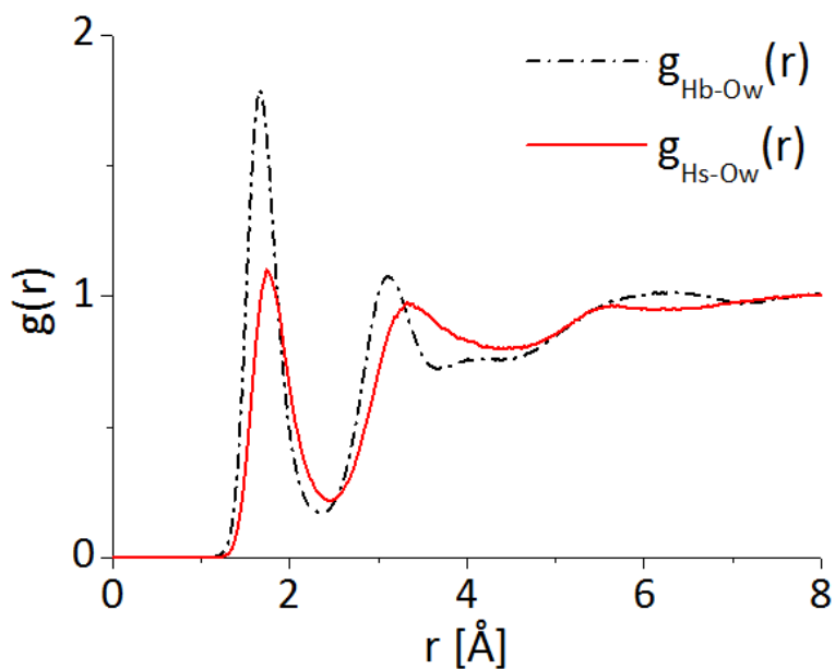
Figure 6. Glutamine – water interactions: Amine-water site-site partial radial distribution functions (RDFs) from the EPSR analysis of neutron diffraction data of the glutamine– water mixture. The g_{Hb-Ow} (dashed, black line) shows the ability of hydrogen atoms on the backbone (Hb) to coordinate water molecules ( O_W ). The g_{Hs-Ow} (solid, red line) shows the ability of hydrogen atoms on the side chain (Hs) to coordinate water molecules ( O_W ).
