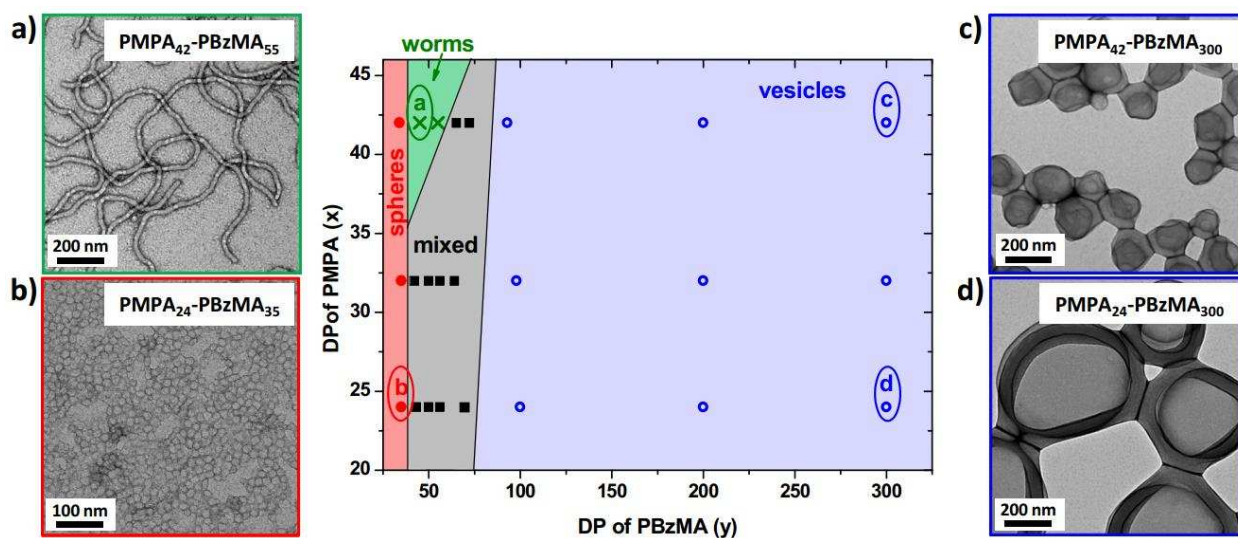
Figure 5. Phase diagram constructed for PMPA x -PBzMA y diblock copolymer nano-objects prepared in methanol at 64 °C at 20% w/w solids. TEM images for pure copolymer morphologies: (a) PMPA 42 -PBzMA 55 (worms), (b) PMPA 24 -PBzMA 35 (spheres), (c) PMPA 42 -PBzMA 300 (small vesicles), and (d) PMPA 24 -PBzMA 300 (large vesicles).
