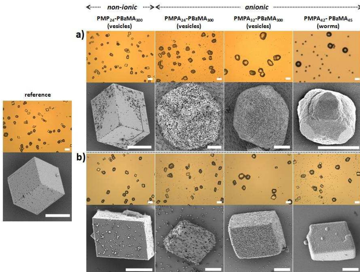
Figure 8. Optical micrographs and corresponding SEM images obtained for a series of CaCO 3 crystals prepared using a 1.5 mM CaCl 2 solution and either (a) 0.010% w/w or (b) 0.005% w/w PMPA-PBzMA or PMP- PBzMA diblock copolymer nano-objects. The scale bar corresponds to 20 \mu m and 5 \mu m for the optical micrographs and SEM images, respectively. Optical micrograph and SEM images of the reference calcite crystals precipitated in the absence of diblock copolymer nano-objects are shown at the left-hand side.
