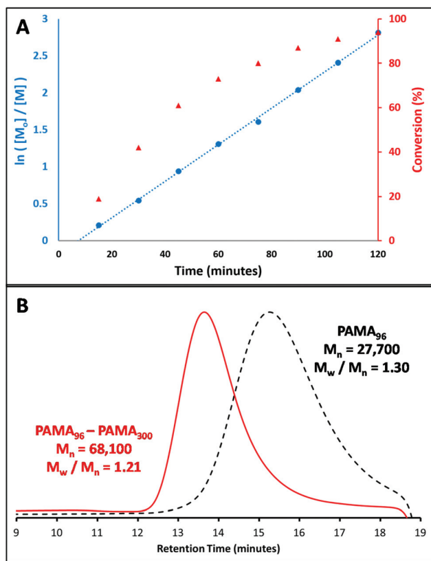
Fig. 2 (A) Conversion vs. time data derived from ^1\text{H} NMR spectroscopy studies of a RAFT solution polymerisation of 2-aminoethyl methacrylate hydrochloride (AMA) at 60^\circ\text{C} in water using MPETTC CTA and AIBA initiator at 20% w/w solids with a CTA/initiator molar ratio = 5. (B) Aqueous gel permeation chromatograms (pH 3.3 vs. PEO standards) obtained for a PAMA 96 macro-CTA, and a subsequent PAMA 300 homopolymer formed by chain extension with further AMA monomer.
