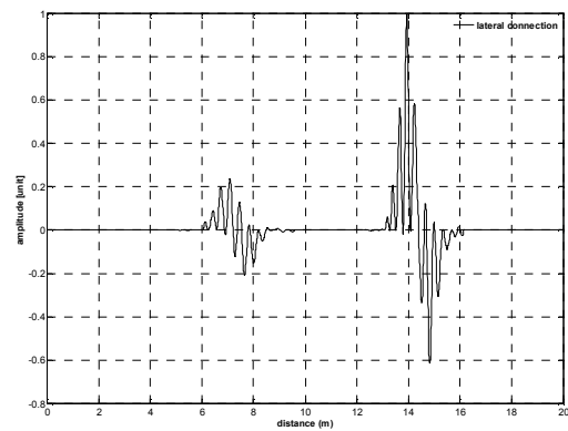
b) Reflection from lateral connection and pipe end of an empty pipe.
