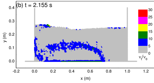
Fig. 4. ISPH computed turbulence viscosity fields
