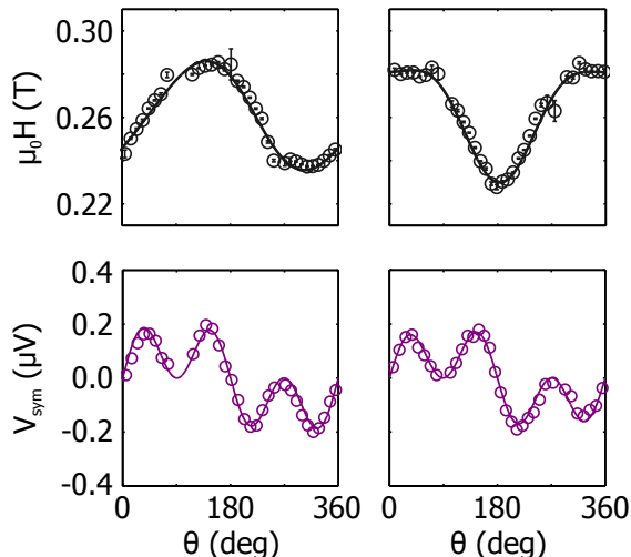
FIG. 5. Independence on the exchange bias direction. Angle dependence of the resonance field for two different 4 nm IrMn bars (top) and corresponding symmetric components of the measured dc voltage (bottom). Although the exchange bias is substantial and has different directions for the two bars, the angle dependence of the symmetric component of the Lorentzian, corresponding to h_z , is not affected.
