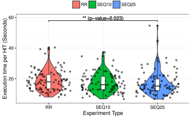
Figure 6: Average Execution time for each HIT submitted from the experimental groups RR, SEQ10 and SEQ25.
