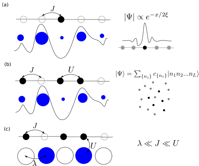
FIG. 1: (Color online) (a) Anderson localization of a single particle hopping on a lattice in the presence of external disorder potential (blue circles). All eigenstates of such a particle in 1D are exponentially localized in space. (b) Many-body localization of particles hopping on a 1D lattice and interacting between nearest neighbour sites. In this case also, the particles move in the background of static external disorder potential (blue circles). For sufficiently strong disorder, the wave function of typical eigenstates is localized (or weakly entangled) in the many-body Fock space. (c) A proposal for MBL in a translation-invariant system, similar to the 1D Hubbard model. In this case, localization is expected to arise dynamically from strong on-site interaction between two species of particles with very different masses ( \lambda \ll J \ll U ), although no external randomness is imposed on the system.
