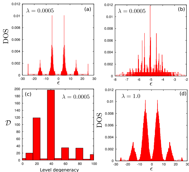
FIG. 2: (Color online) The DOS for the model (2) and separation into non-overlapping bands for L = 10 , U = 10 , J = 1 .
