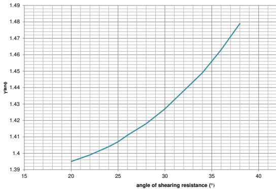
Figure 13. \gamma_{\tan\phi'} for different values of angle of shearing resistance
