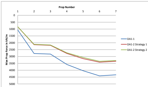
Figure 9. Maximum prop loads from different factoring strategies using HS soil model
