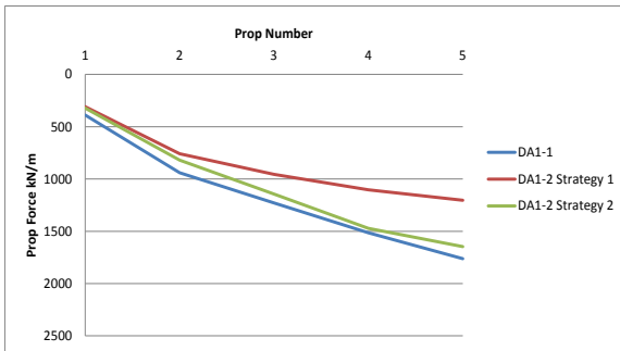
Figure 4. Maximum prop loads from different factoring strategies using MC soil model
