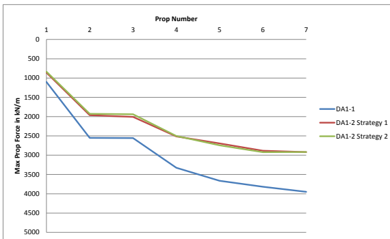
Figure 10. Maximum prop loads from different factoring strategies using HSS soil model
