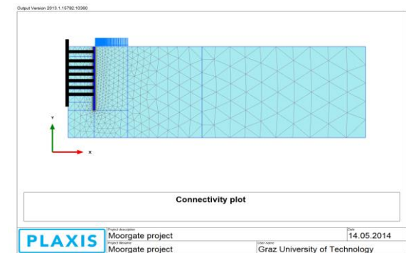
Figure 7. Finite Element mesh
