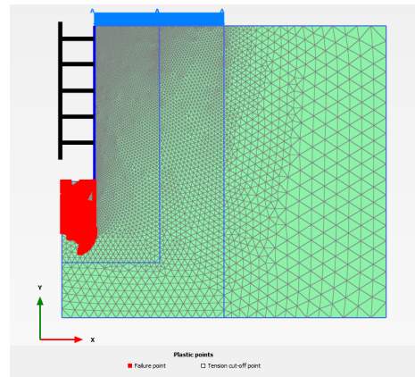
Figure 3. Plastic points developed at the final excavation stage
