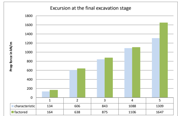
Figure 2. Prop loads before and after factoring soil strength in Strategy 2 at the final excavation stage
