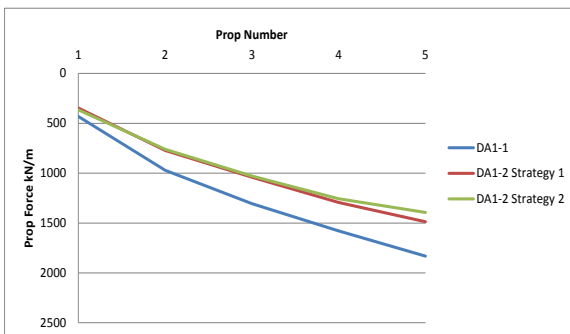
Figure 6. Maximum prop loads from different factoring strategies using HSS soil model
