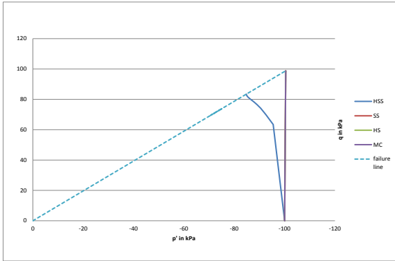
Figure 12. p-q stress paths using different soil models
