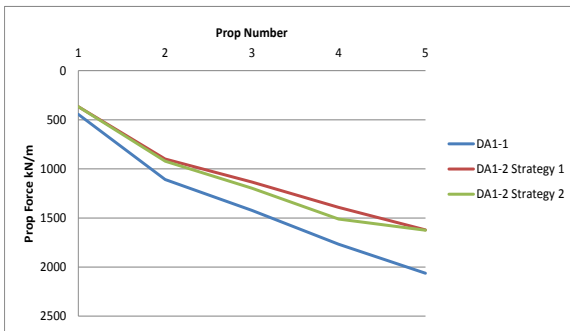
Figure 5. Maximum prop loads from different factoring strategies using HS soil model
