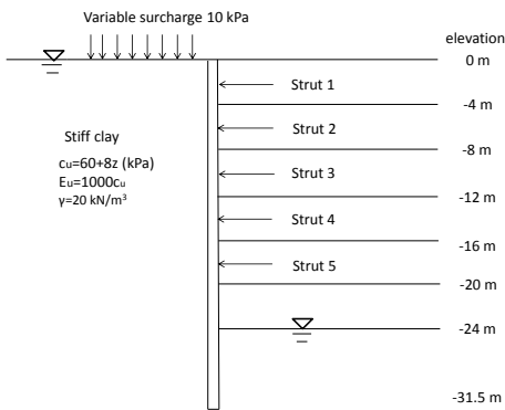
Figure 1. Geometry of deep excavation supported by 5 levels of props
