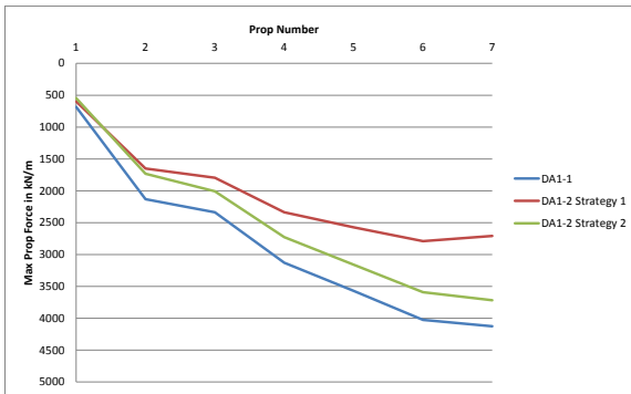
Figure 8. Maximum prop loads from different factoring strategies using MC soil model
