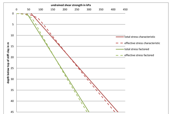
Figure 11. Characteristic and design undrained shear strength profiles using total and effective stress MC, HS and HSS parameters
