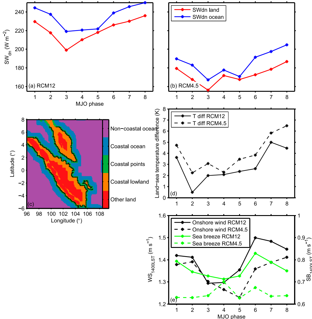
FIG. 11. Mean surface SW_{dn} radiative flux by MJO phase for (a) RCM12 and (b) RCM4.5. (c) The coastal ocean (blue) and coastal lowland (orange) classification used to compute the land–ocean temperature difference, and the coastal points (black dots) used to compute the onshore wind speeds and sea breeze for RCM12. Coastal is defined as within 120 km of the coastline and lowland as 500 m below mean sea level. Note that a number of the smaller islands have been removed for this analysis. (d) The surface temperature difference at 1400 LST between coastal lowland and coastal ocean; (e) the mean onshore 10-m wind speed ( WS_{1400LST} , black lines) and the mean 10-m sea breeze ( SB_{1400LST} , green lines), both by MJO phase at 1400 LST.
