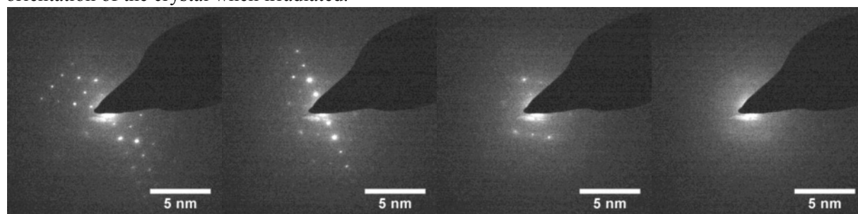
Figure 2: Diffraction pattern series of indapamide initially oriented on the [110] zone axis with electron flux of 3.59 \text{ electrons nm}^{-2} \text{ s}^{-1} at 45, 120, 170 and 250 seconds after initial exposure to the electron beam. The pattern changes to a systematic row after 120s before fading, consistent with a change in orientation of the crystal as well as a decrease in crystallinity.
