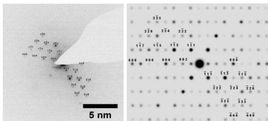
Figure 1: (a) Electron diffraction pattern from an indapamide crystal oriented close to the [110] zone axis, recorded with an electron flux of 3.59 \text{ electrons nm}^{-2} \text{ s}^{-1} (b) [110] pattern simulation using CrystalMaker software and indapamide structure listed in Table 1.
