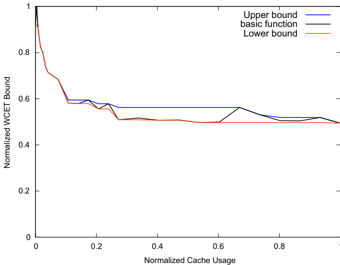
Fig. 3 Over-/underapproximations of the WCET function ( stateate benchmark, direct mapped data cache, perfect instruction cache)
