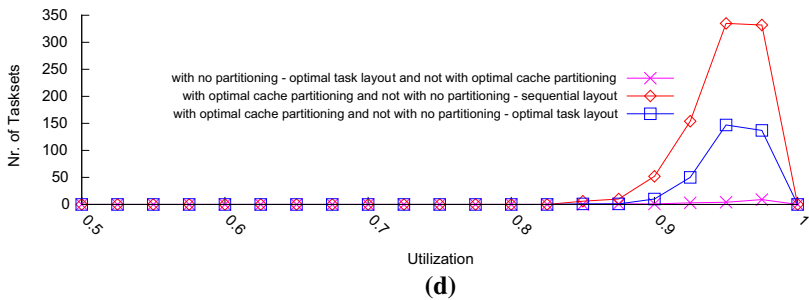
Fig. 5 Evaluation of PapaBench benchmarks (fixed priority scheduling). a Number of tasksets deemed schedulable at the different total utilizations (instruction cache with perfect data cache), b number of tasksets deemed schedulable with one approach and not another (instruction cache with perfect data cache), c number of tasksets deemed schedulable at the different total utilizations (data cache with perfect instruction cache), d number of tasksets deemed schedulable with one approach and not another (data cache with perfect instruction cache)
