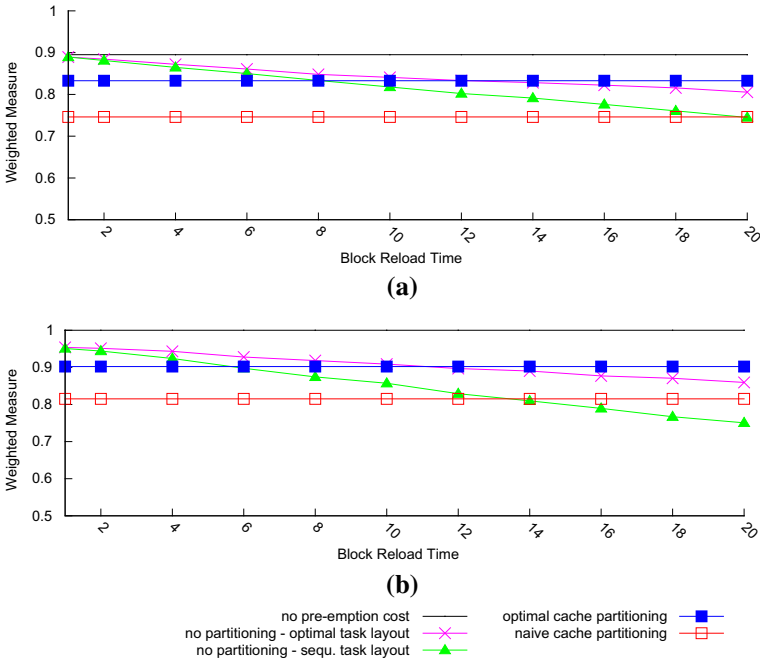
Fig. 15 Weighted schedulability measure; varying block reload time from 1 to 20 μs (assuming constant worst-case execution times). a Fixed priority scheduling, b EDF scheduling
