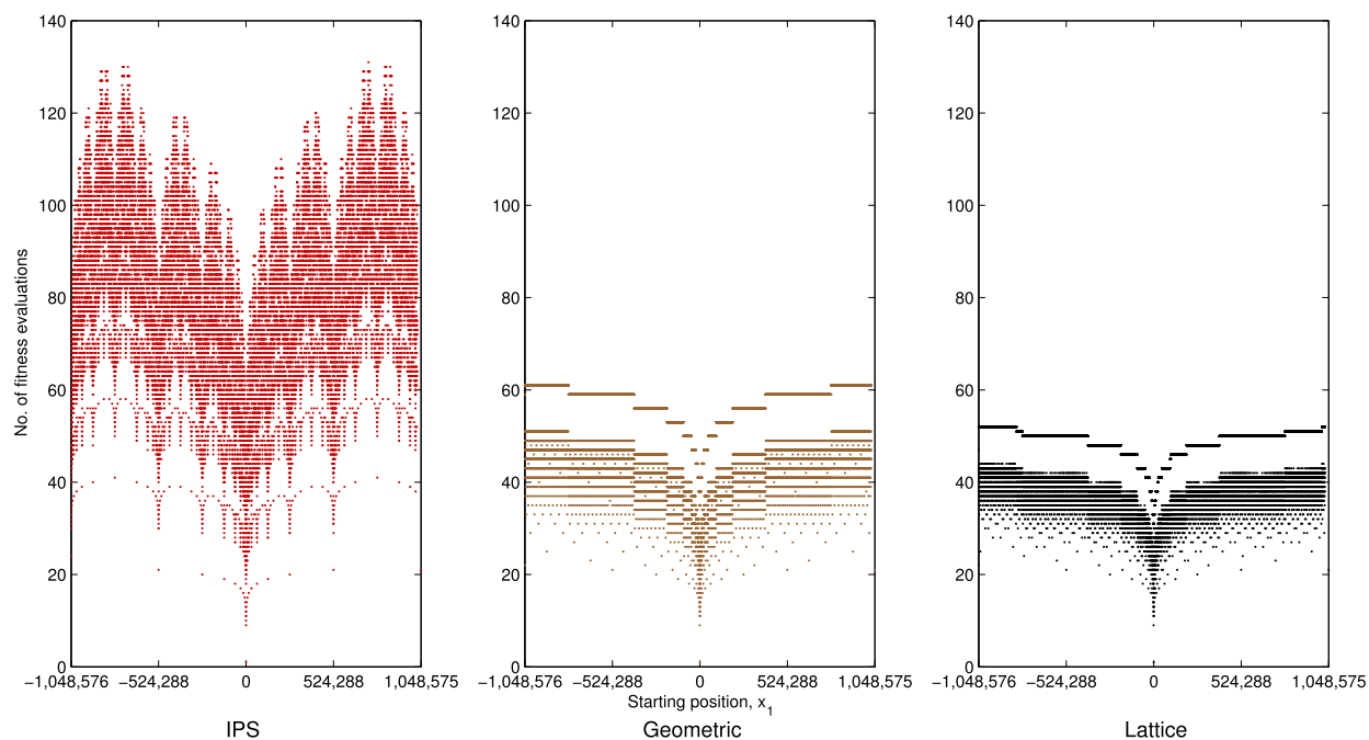
Fig. 4. Number of unique fitness evaluations for optimizing f(x) = |x| with different local searches for each starting position x_1 \in [-2^{20}, 2^{20} - 1] . For the sake of clarity, the plots do not show all 2^{21} data points, but were downsampled to a selection of 25 000 data points for each search to give a good and accurate visual representation of all 2^{21} points, using the Largest-Triangle-Three-Buckets algorithm [27].
