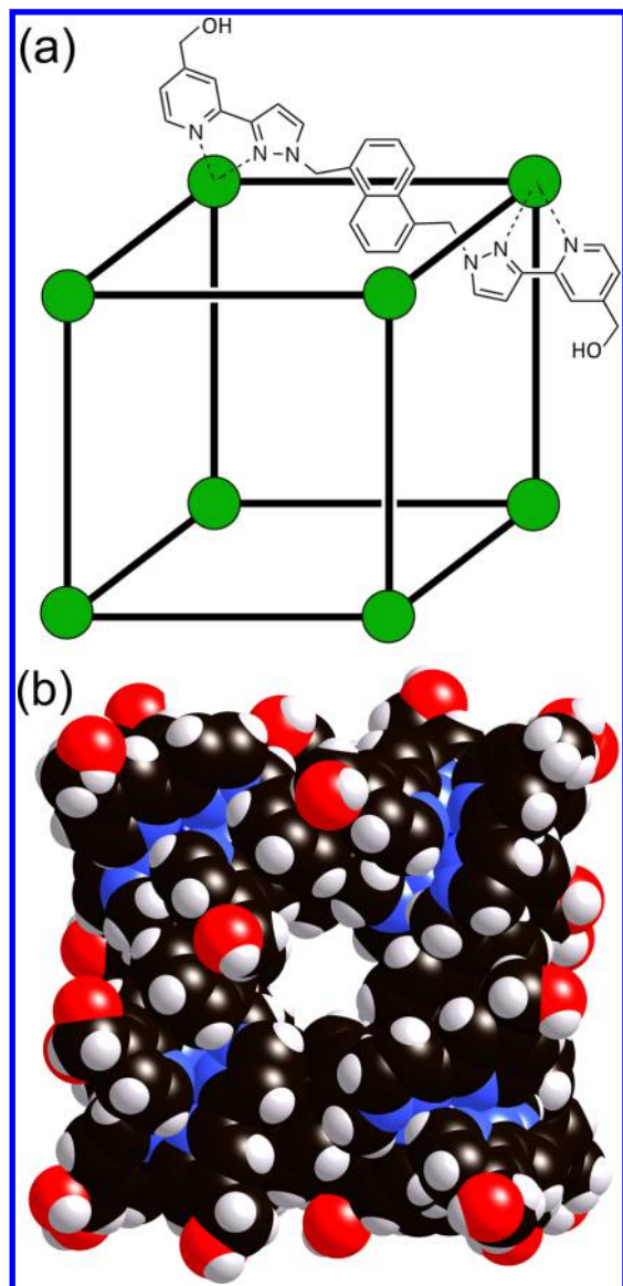
Figure 1. Structure of the host cage [\text{Co}_8\text{L}_{12}](\text{BF}_4)_{16} . (a) Sketch of the octanuclear core showing the disposition of the bridging ligands. (b) Space-filling view of the complete cage cation, showing the external O atoms of the hydroxyl groups in red. Panel (b) is reproduced with permission from ref 13. Copyright 2013 Royal Society of Chemistry.
