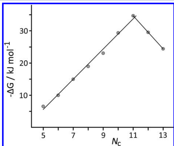
Figure 4. Plot of binding free energy vs number of C atoms for guest series A. The best-fit straight lines to the data points for N_C = 5 –11 (rising: -\Delta G / \text{kJ mol}^{-1} = 4.7N_C - 18.1 ; R^2 > 0.99 ) and N_C = 11 –13 (descending) are included.
