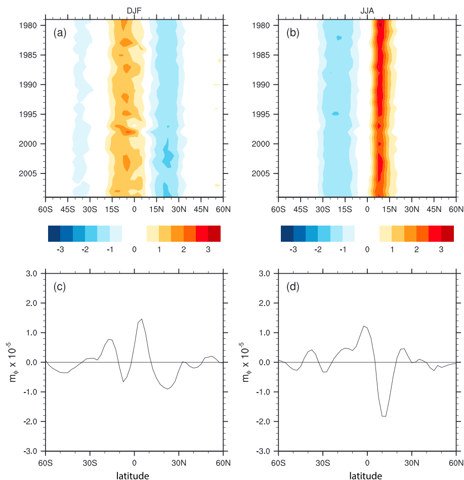
Figure 13. (a, b) The zonally averaged ( 0\text{--}360^\circ ) meridional vertical mass flux at 500 hPa averaged over ERAI, NCEP2, MERRA, and JRA reanalyses between 1979 and 2009 ( \times 10^{-3} \text{ kg m}^{-2} \text{ s}^{-1} ) for the seasons DJF and JJA. (c, d) The averaged trend in the zonally averaged meridional mass flux ( \times 10^{-5} \text{ kg m}^{-2} \text{ s}^{-1} over 31 years).
