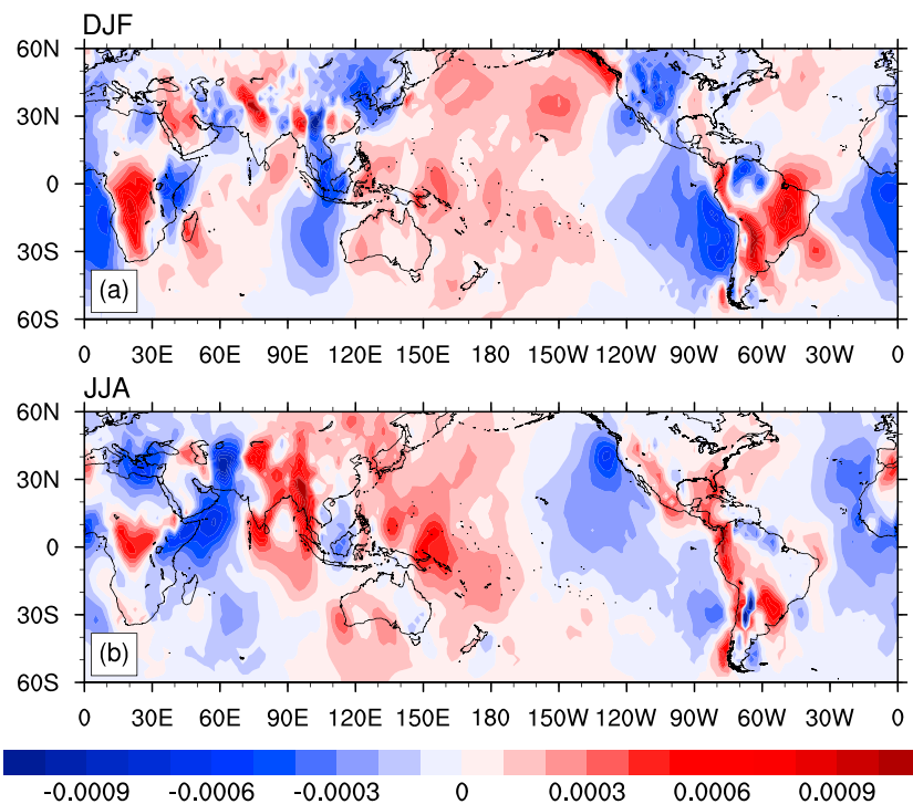
Figure 5. The local Walker circulation. The zonal mass flux ( \text{kg m}^{-2} \text{s}^{-1} ) for the seasons (a) DJF and (b) JJA is shown in shadings of red (ascent) and blue (descent) at 500 hPa and are averaged over ERAI, NCEP2, MERRA, and JRA reanalyses (1979–2009).
