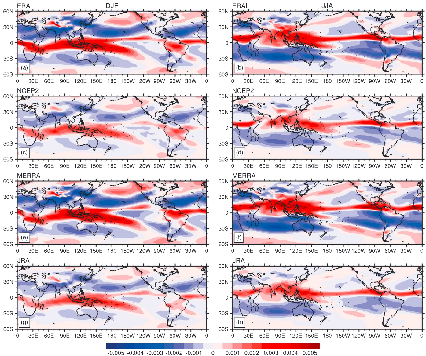
Figure 6. The meridional mass flux ( \text{kg m}^{-2} \text{s}^{-1} ) for the seasons DJF and JJA averaged over the period 1979–2009 are shown in shadings of red (ascent) and blue (descent) at 500 hPa for the reanalyses (a, b) ERAI, (c, d) NCEP2, (e, f) MERRA, and (g, h) JRA.
