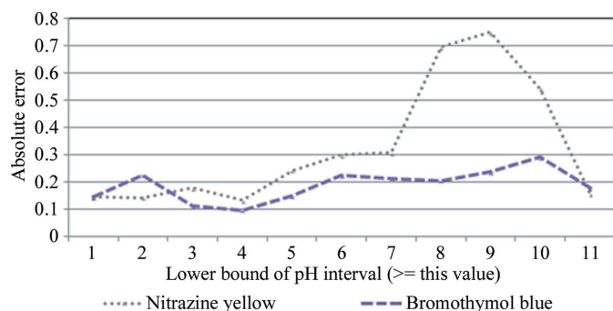
Figure 4 The mean errors between the measured pH and the values calculated with the spectrophotometric method using the indicator dyes nitrazine yellow and bromothymol blue. The errors are given as absolute values averaged over 0.5 pH unit bins (as determined by the pH meter readings). It can be seen that the errors are significantly worse for nitrazine yellow for pH 8.0–10.0.
