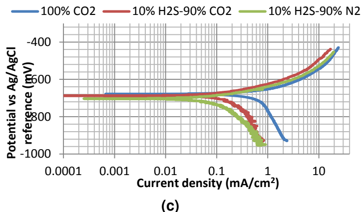
Figure 1. Tafel polarization plots for UNS K03014 carbon steel in 3.5 wt.% NaCl solution saturated with 100 mol.% CO 2 , 10 mol.% H 2 S- 90 mol.% CO 2 and 10 mol.% H 2 S-90 mol.% N 2 at (a) 30°C, (b) 50°C and (c) 80°C.
