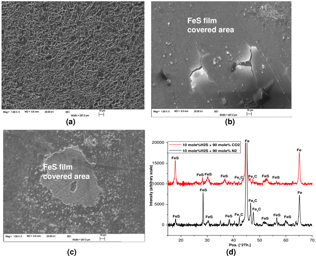
Figure 5: SEM images of corrosion product layer on UNS K03014 carbon steel in 3.5 wt. % NaCl solution saturated with (a) 100 mol. % CO 2 , (b) 10 mol. % H 2 S- 90 mol. %CO 2 and (c) 10 mol. % H 2 S- 90 mol. % N 2 at 50°C. (d) XRD pattern for corrosion product layer on UNS K03014 carbon steel in 3.5 wt.% NaCl solution saturated 10 mol. % H 2 S- 90 mol. %CO 2 and 10 mol. % H 2 S-90 mol. % N 2 at 50°C. Images are for test duration of 7 hours. (Note that the intensity scale is arbitrary).
