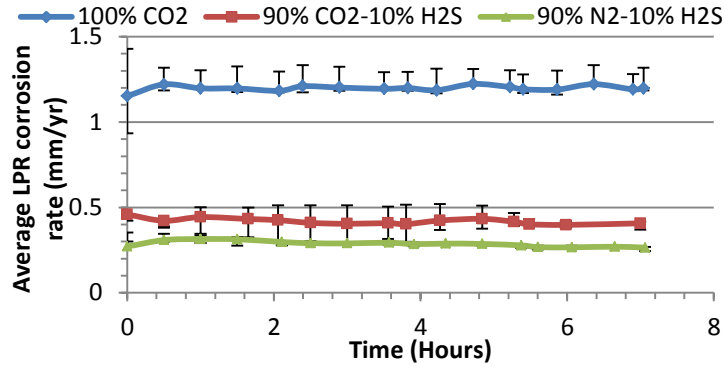
Figure 2. Corrosion rate of UNS K03014 carbon steel in 3.5 wt.% NaCl solution saturated with gas streams of different composition at 30°C.
