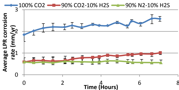
Figure 4: Corrosion rate of UNS K03014 carbon steel in 3.5 wt.% NaCl solution saturated with gas streams of different composition at 50°C.
