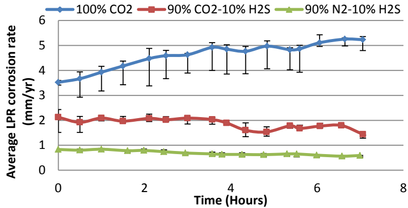
Figure 6: Corrosion rate of UNS K03014 carbon steel in 3.5 wt.% NaCl solution saturated with gas streams of different composition at 80°C.
