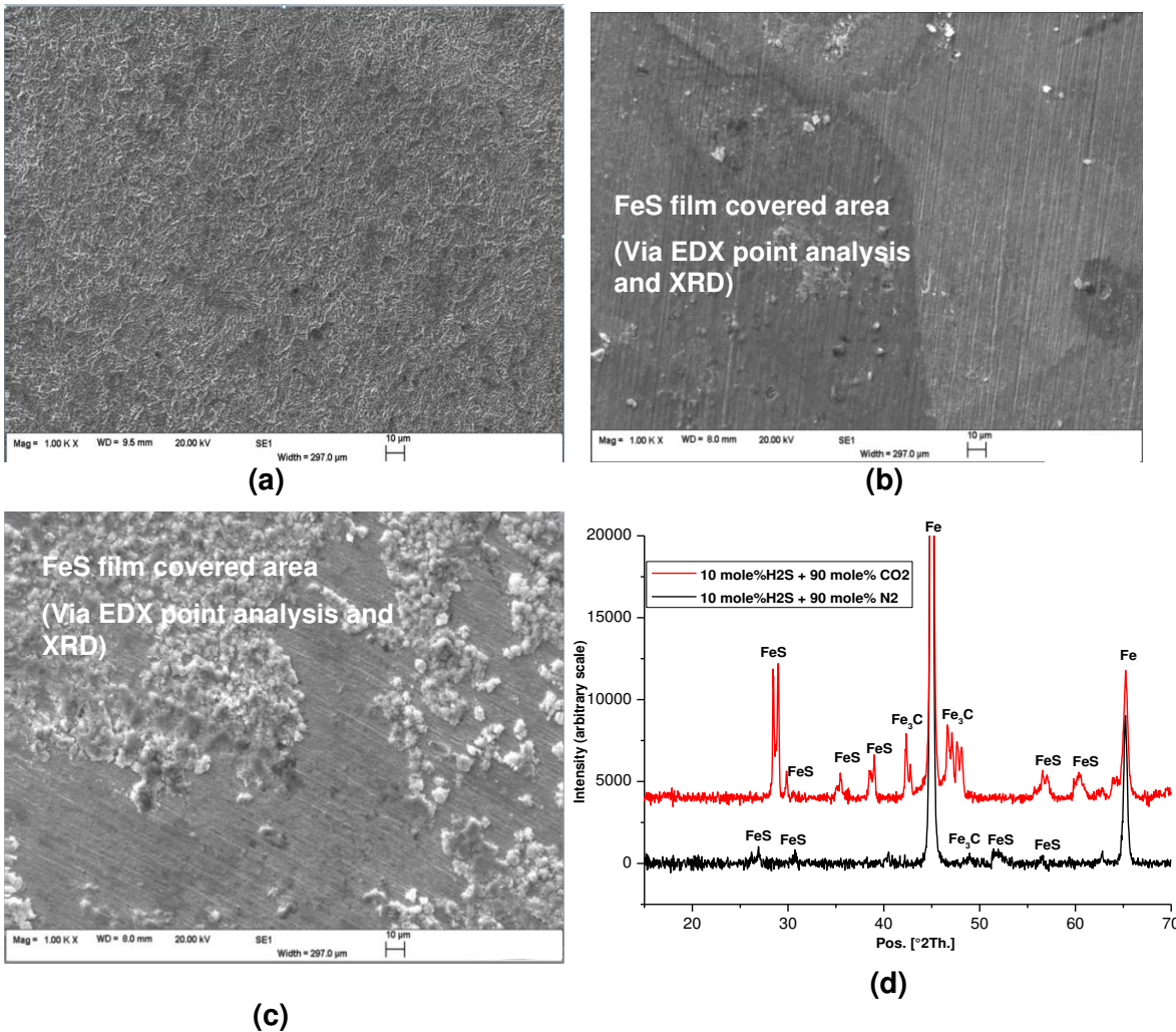
Figure 3: SEM images of corrosion product layer on UNS K03014 carbon steel in 3.5 wt. % NaCl solution saturated with (a) 100 mol. % CO 2 , (b) 10 mol. % H 2 S- 90 mol. % CO 2 and (c) 10 mol. % H 2 S- 90 mol. % N 2 at 30°C. (d) XRD pattern for corrosion product layer on UNS K03014 carbon steel in 3.5 wt.% NaCl solution saturated 10 mol. % H 2 S- 90 mol. % CO 2 and 10 mol. % H 2 S-90 mol. % N 2 at 30°C. Images are for test duration of 7 hours. (Note that the intensity scale is arbitrary).
