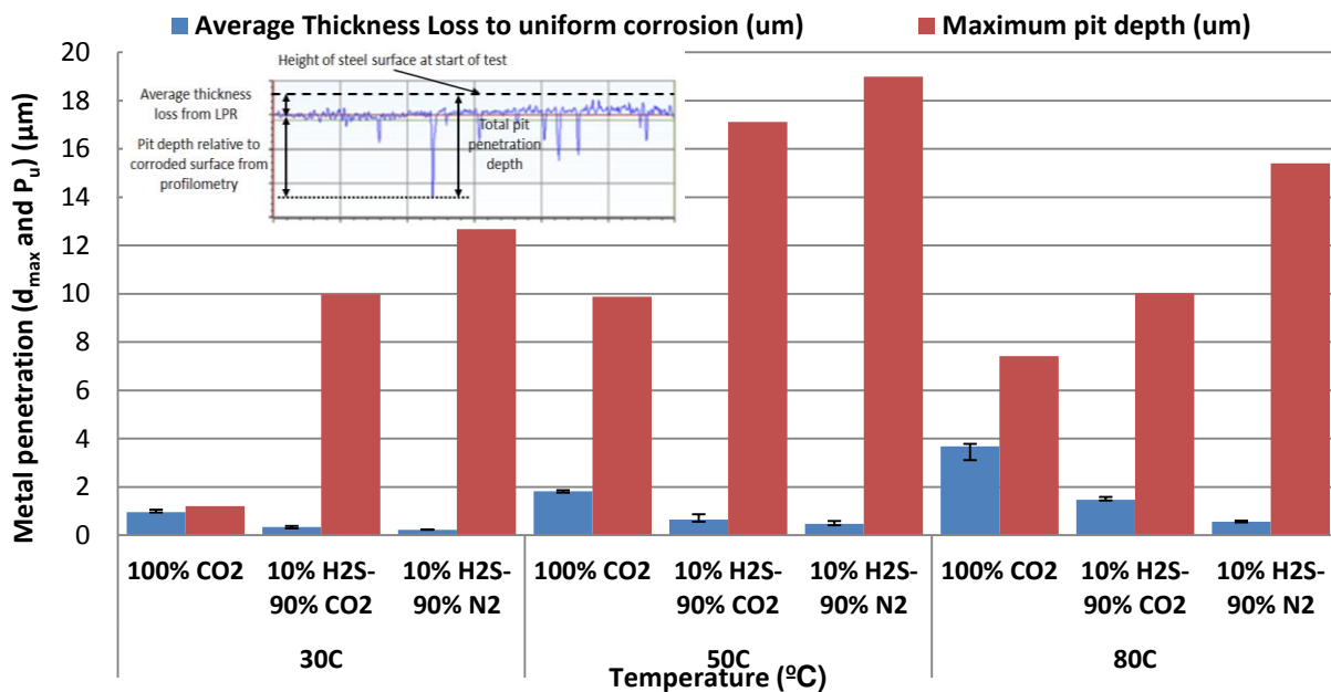
Figure 10: Total pit penetration on UNS K03014 carbon steel surface exposed to corrosion system under 100mol.% CO 2 , 10mol.% H 2 S - 90mol.% CO 2 and 10mol.% H 2 S - 90mol.% N 2 gas atmosphere as a function of temperature indicating the contribution of general thickness loss (from LPR) and pit depth relative to corroded surface (determined from surface profilometry)
