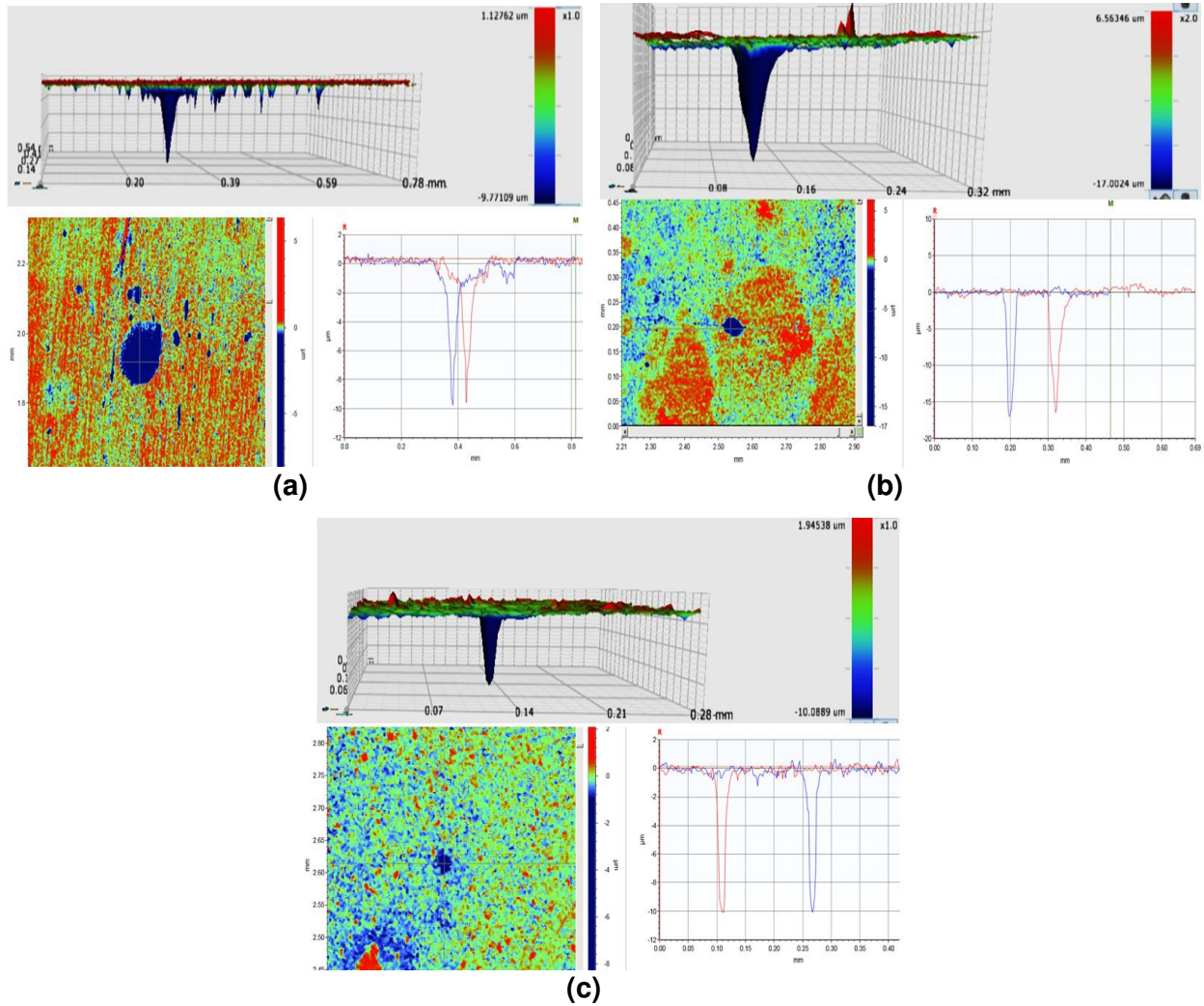
Figure 9: 2D and 3D images of Deepest pit (relative to corroded surface) on UNS K03014 carbon steel surface exposed to corrosion system under 10mole% H 2 S - 90mole% CO 2 for 7 hours at (a) 30°C, (b) 50°C, and (c) 80°C.
