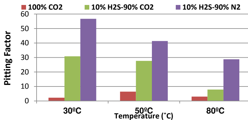
Figure 11: Variation of pitting factor for UNS K03014 carbon steel surface exposed to corrosion system under 100mole% CO 2 , 10mole% H 2 S - 90mole% CO 2 and 10mole% H 2 S - 90mole% N 2 gas atmosphere as a function of temperature.
