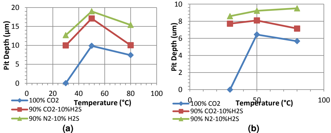
Figure 8: (a) Maximum pit depth (relative to corroded surface) and (b) Average pit depth (relative to corroded surface) on UNS K03014 carbon steel surface exposed to corrosion system under 100mol. % CO 2 , 10mol. % H 2 S - 90mol. % CO 2 and 10mol. % H 2 S - 90mol. % N 2 gas atmosphere as a function of temperature.
