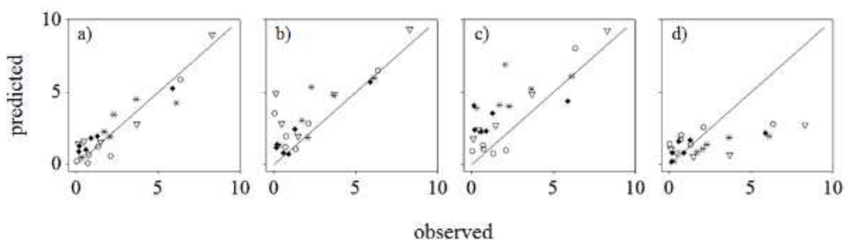
Fig. 7. Predicted versus observed values for mean earthworm population biomass ( \text{g/m}^2 ) responses to carbendazim in the three German (G1:▽, G2:◆, G3:○) and one Spanish (S2:*) field trial/s for a) the presented model ( R^2 = 0.92 ), b) for when pesticide effects on mortality are removed ( R^2 = 0.68 ), c) when aestivation due to dry soil conditions is excluded ( R^2 = 0.51 ), and d) when movement is assumed to be random ( R^2 = 0.50 ).
