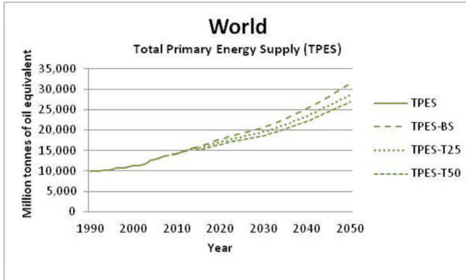
31 Figure 2 Global total primary energy supply (TPES, in Mtoe), 1990 to 2050; historical data and 32 three scenario projections
