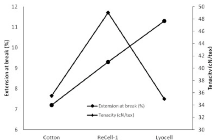
Fig. 6. Comparison of extension at break (C) and tenacity (A) of ReCell, Lyocell and cotton fibres. The cotton figure values are literature-based (Cook, 1984; Bredereck and Hermanutz, 2005; Woodings, 1995; Taylor, 1998).
