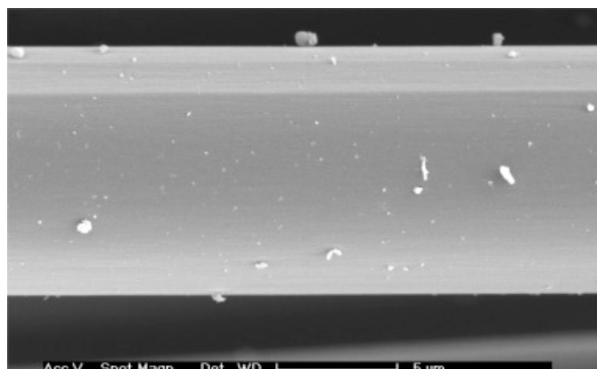
Fig. 1. SEM micrograph of Lyocell fibres at 5000_ magnification and an accelerating voltage of 5 kV.
