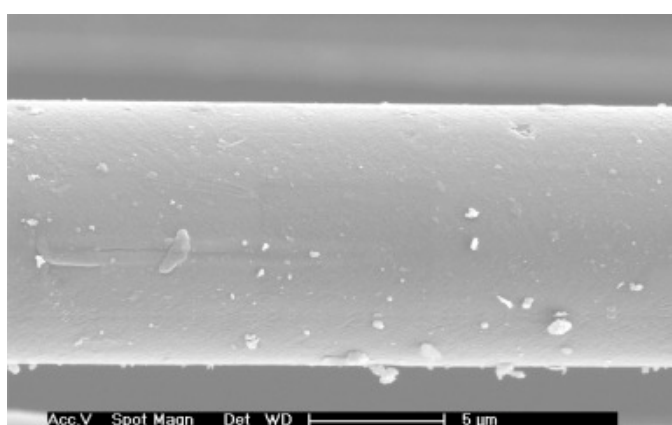
Fig. 4. SEM micrograph of ReCell-1 fibres at 5000_ magnification and an accelerating voltage of 5 kV.
