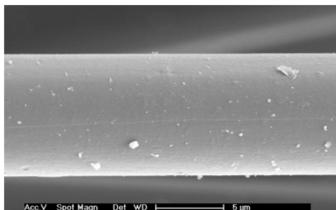
Fig. 2. SEM micrograph of ReCell-Denim fibres at 5000_ magnification and an accelerating voltage of 5 kV.
