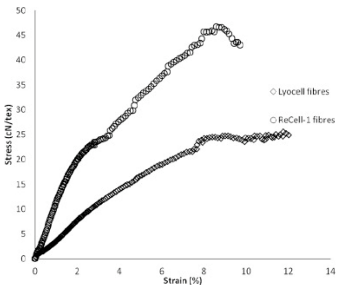
Fig. 5. Stress/strain curves for Lyocell and ReCell-1 fibres (each 1.33 dtex).
