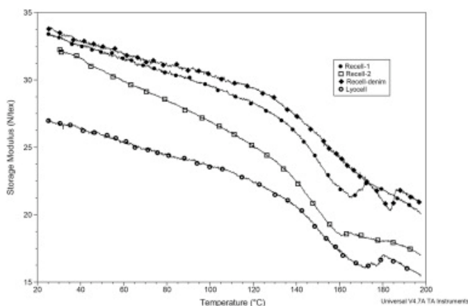
Fig. 7. Storage modulus of A-ReCell-Denim, C-ReCell-1, -ReCell-2 and B-Lyocell fibres with increasing temperature.
