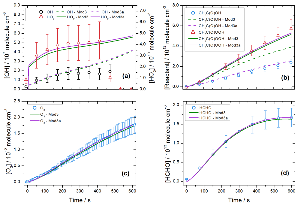
Figure 7. Experimental results for OH and HO 2 , (a) , CH 3 C(O)OOH and CH 3 C(O)OH, (b) , O 3 , (c) and HCHO, (d) , as a function of time for experiment P9 where [CH 3 OH] 0 : [CH 3 CHO] 0 = 0.0, 1000 mbar and 293 K. Yields for Reaction (R5) were modelled using the base model reaction scheme shown in Table 2 and varied to fit the measurements, using k_{(R5)} = (2.4 \pm 0.4) \times 10^{-11} \text{ cm}^3 \text{ molecule}^{-1} \text{ s}^{-1} and \alpha_{(R5a)} = 0.42 \pm 0.05 , \alpha_{(R5b)} = 0.14 \pm 0.04 and \alpha_{(R5c)} = 0.44 \pm 0.10 (Model3). Model agreement to measured CH 3 C(O)OH was improved by varying the modelled branching ratios of Reactions (R20a) and (R20b) are shown in trace Model3a. All uncertainties quoted to \pm 2\sigma .
