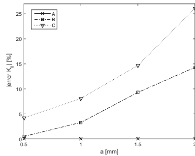
Fig. 13 The absolute relative error for mode-II |error K_{II}| (%) is represented against the half-crack length a for geometries A,B and C.
