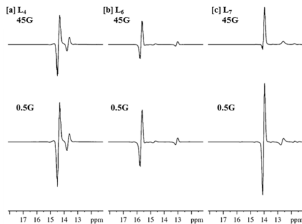
Figure 4 SABRE hyperpolarized 31 P NMR traces for L 4 [a], L 6 [b] and L 7 [c] that result after polarization transfer catalysis in a 45 G or 0.5 G field.
