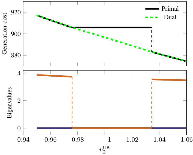
Fig. 8. Performance of SDP optimization method on 2-bus problem.
