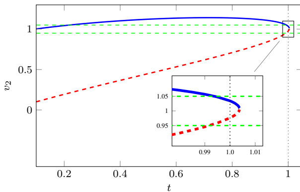
Fig. 2. Alternate load flow solutions as the demand parameter, t , varies.
