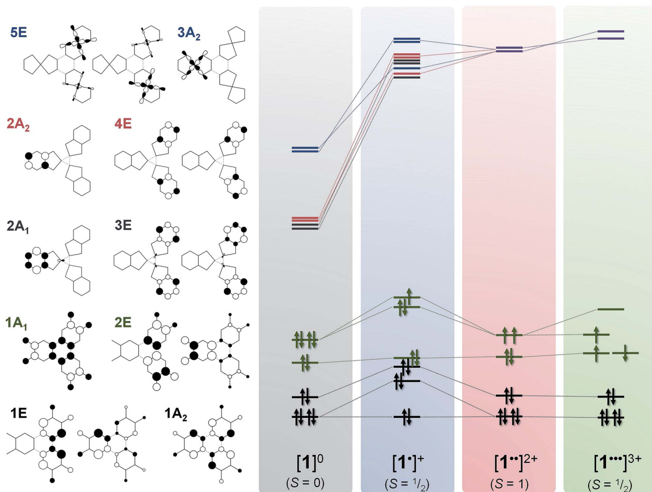
Fig. 9 Qualitative MO scheme depicting the ordering of frontier orbitals for the [1]^{0/1+2+3+} electron transfer series, derived from B3LYP-ZORA DFT calculations. The idealised orbitals shown left are derived from the calculation of 1 annotated with C_{3v} symmetry labels. The purple levels represent mixing of 2A_2 and 4E (red) with 3A_2 and 5E (blue). Detailed schemes and MO plots are in Fig. S25–S28†.
