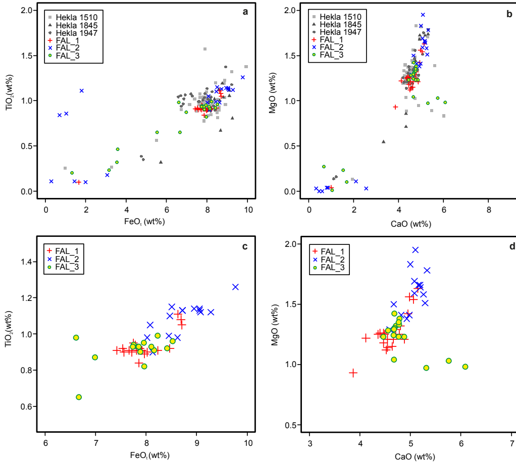
Fig. 6. Tephra geochemistry co-variation diagrams for (a–b) full range of FeO_1 (wt%), TiO_2 (wt%), CaO (wt%), MgO (wt%) values for the three tephra horizons in core A at Fallahogy plotted against type data for the Hekla eruptions of 1510, 1845 and 1947 from TephraBase (Newton et al., 2007). (c–d) a restricted range of FeO_1 (wt%), TiO_2 (wt%), CaO (wt%), MgO (wt%) values for the three tephra horizons in core A at Fallahogy to show in more detail the overlap between the geochemical distributions, all data are normalised.
