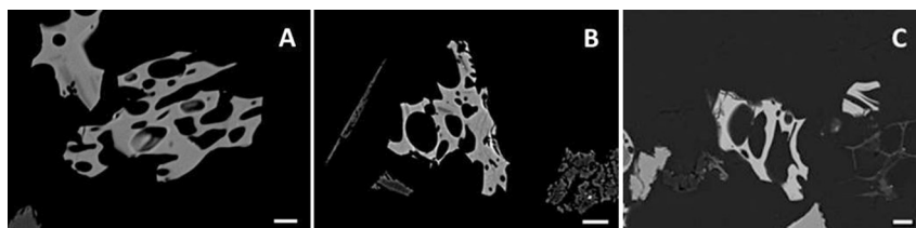
Fig. 4. Scanning electron microscope images of typical tephra shards exposed for geochemical analysis (a) Hekla 1510 (b) Hekla 1845 (c) Hekla 1947. White scale bars are 10 µm.
