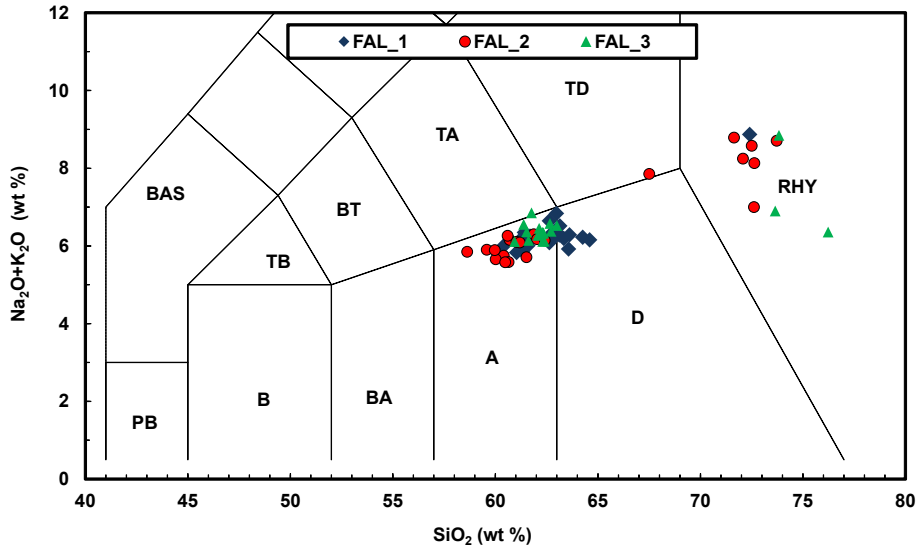
Fig. 5. Total Alkali Silica (TAS) Diagram showing the three tephras detected in core A at Fallahogy (raw data). Shards are mainly of andesitic-dacitic geochemistry. Annotations follow standard terminology e.g. RHY = Rhyolite, D = Dacite, A = Andesite (Le Maitre et al., 1989).
