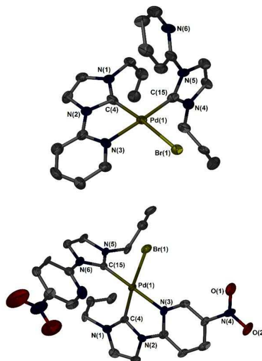
Fig. 1 Molecular structure of complexes 3a (top) and 3c (bottom). Ellipsoids are shown at the 50% probability level, hydrogen atoms, bromide counter anions and solvent molecules ( 3a : one molecule of MeOH; 3c : one molecule of MeOH) are omitted for clarity. Selected bond distances (Å) and angles (°): 3a Pd1–C4 1.961(12), Pd1–C15 1.968(10), Pd1–Br1 2.4542(13), Pd1–N3 2.091(8), N3–Pd1–C4 79.6(4), Br1–Pd1–C4 175.1(3). 3c Pd1–C4 1.994(9), Pd1–C15 1.978(8), Pd1–Br1 2.4508(12), Pd1–N3 2.090(7), N3–Pd1–C4 79.0(3), Br1–Pd1–C4 174.1(3).
