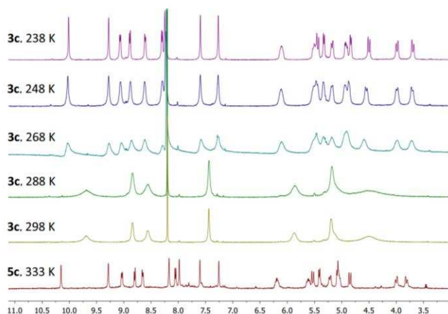
Fig. 4 VT 1 H NMR spectra (500 MHz, CD 3 CN) of Pd II -bis-NHC complexes 3c (238 – 298 K) and 5c (333 K).
