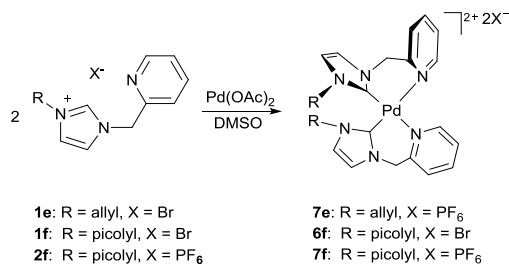
Scheme 4 Preparation of picolyl-substituted Pd II -bis-NHC complexes 7e , 6f and 7f .
