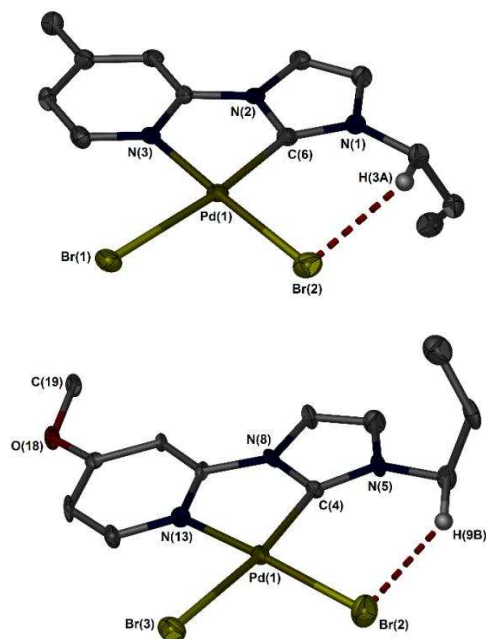
Fig. 2 Molecular structure of complexes 4b (top) and 4d (bottom). Ellipsoids are shown at the 50% probability level, hydrogen atoms (except H3A and H9B) are omitted for clarity. Selected bond distances (Å) and angles (°): 4b Pd1–C6 1.982(4), Pd1–Br1 2.4820(5), Pd1–Br2 2.4266(5), Pd1–N3 2.065(3), N3–Pd1–C6 79.83(14), Br1–Pd1–C6 172.47(11). 4d Pd1–C4 1.998(8), Pd1–Br2 2.4175(11), Pd1–Br3 2.4703(10), Pd1–N13 2.057(7), N13–Pd1–C4 80.3(3), Br3–Pd1–C4 171.9(2).
