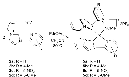
Scheme 3 Preparation of Pd II - bis -NHC dihexafluorophosphate complexes 5a-5d .
