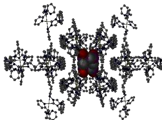
Fig. 7 Molecular structure of complex 6f (top), space-filling diagram revealing a solvent-accessible pore running parallel to the crystallographic c axis (middle), and ball-and-stick diagram with space-filled model of four DMSO molecules occupying one accessible channel (bottom). Ellipsoids are shown at the 50% probability level, hydrogen atoms, bromide counter anions and solvent molecules ( 6f (top): one molecule of DMSO, only those modelled are shown below) are omitted for clarity. Selected bond distances (Å) and angles (°): Pd1–C7 1.964(8), Pd1–C22 1.980(7), Pd1–N4 2.109(6), Pd1–N8 2.103(7), N4–Pd1–C7 85.1(3), N8–Pd1–C22 85.4(3), C7–Pd1–N8 179.5(3), C22–Pd1–N4 175.5(3).
