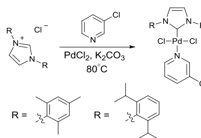
Scheme 1 Synthetic route to Pd-PEPPSI catalysts. 28,29
