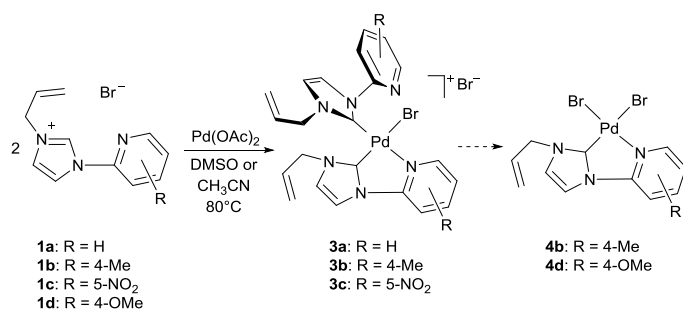
Scheme 2 Preparation of \text{Pd}^{\text{II}} - bis -NHC dibromide complexes 3a–3c and \text{Pd}^{\text{II}} - mono -NHC dibromide complexes 4b and 4d .
