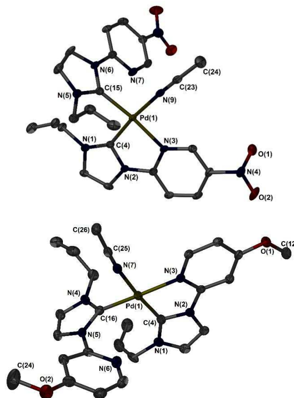
Fig. 3 Molecular structure of complexes 5c (top) and 5d (bottom). Ellipsoids are shown at the 50% probability level, hydrogen atoms and hexafluorophosphate counter anions are omitted for clarity. Selected bond distances (Å) and angles (°): 5c Pd1–C4 1.962(3), Pd1–C15 1.978(3), Pd1–N9 2.055(2), Pd1–N3 2.092(2), N3–Pd1–C4 80.25(10), N9–Pd1–C4 172.81(10). 5d Pd1–C4 1.964(4), Pd1–C16 1.989(4), Pd1–N3 2.078(3), Pd1–N7 2.059(4), N3–Pd1–C4 79.63(14), N7–Pd1–C16 91.24(15), C4–Pd1–C16 95.71(16), C4–Pd1–N7 172.42(15), C16–Pd1–N3 171.86(15).
