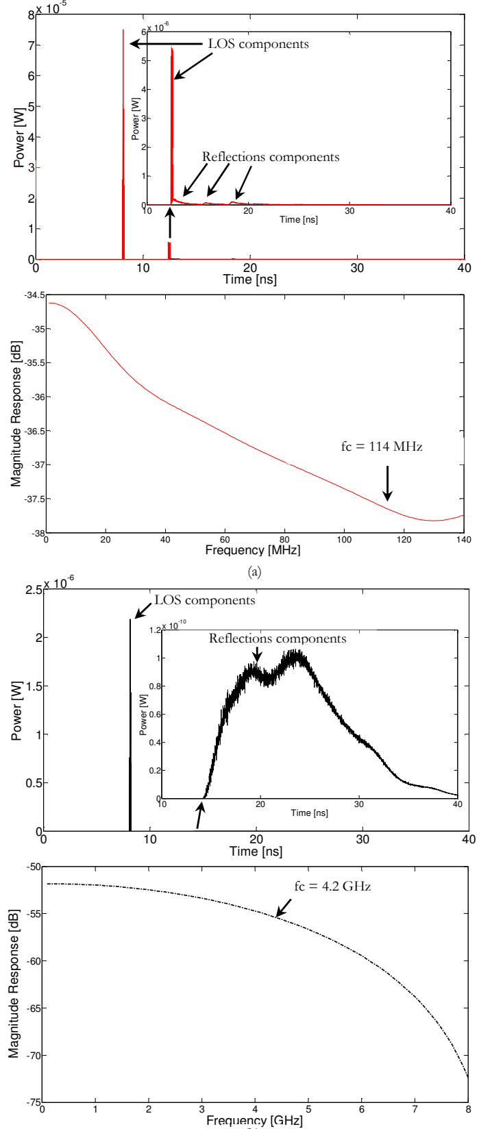
Fig.7: Impulse and frequency responses of the two receivers, (a) wide FOV receiver (b) imaging receiver at room centre ( x=2\text{m} , y=4\text{m} , z=1\text{m} ).
