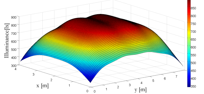
Fig.3: Distribution of horizontal illumination at the communication floor, Min. 336 lx and Max. 894 lx.
