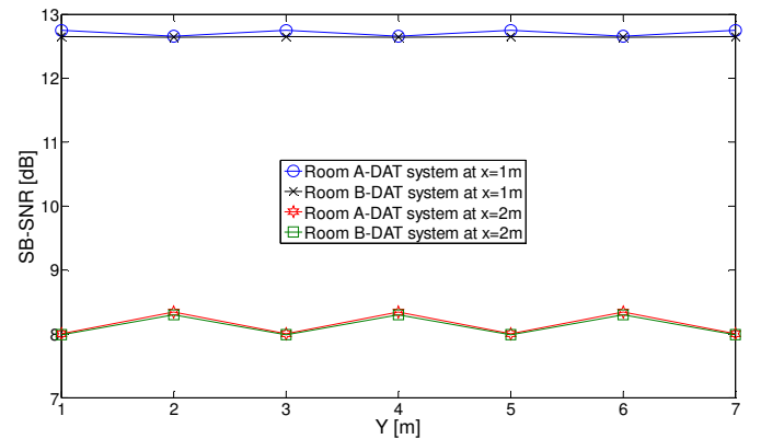
Fig.19: SB-SNR of DAT system in two different environments (rooms A and B) when system operated at 10 Gbps at x=1\text{m} and x=2\text{m} along y -axis.
