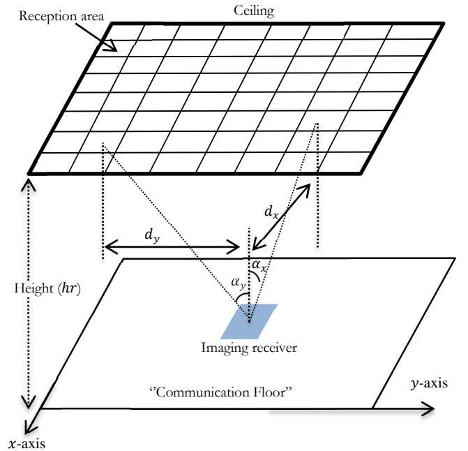
Fig.5: Reception area distribution associated with the photo-detector array when the receiver is placed at the centre of the room.
