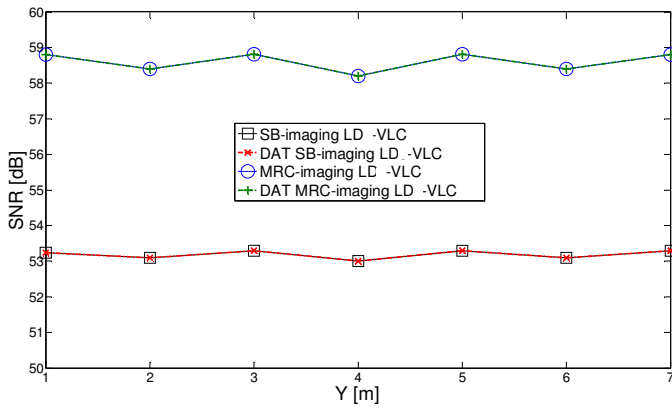
Fig.14: SNR of imaging system and DAT imaging system when both operate at 30 Mbps, when the receivers move at x=2m and along y -axis.
