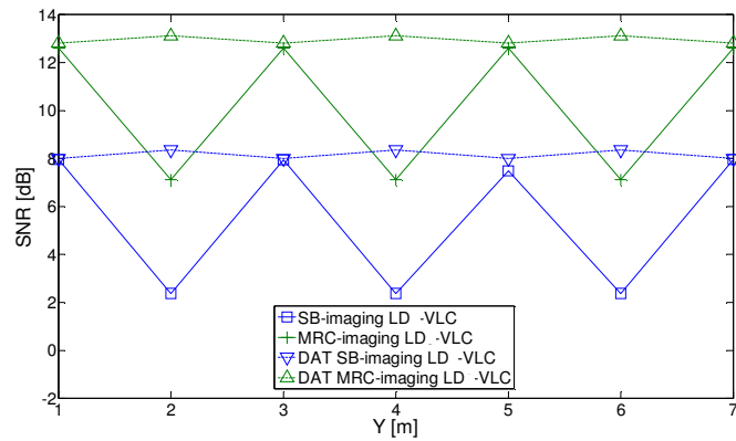
Fig.15: SNR of imaging system and DAT imaging system when both operate at 10 Gbps, when the receivers move at x=2m and along y -axis.
