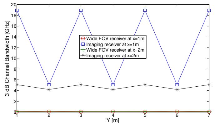
Fig.9: 3 dB channel bandwidth of the wide FOV and the imaging LD-VLC systems in fourteen different locations when all the receivers move along the y-axis.
