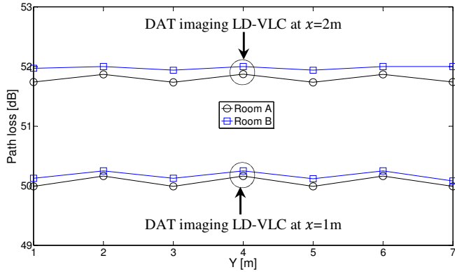
Fig.17: Optical path loss distribution of the DAT imaging system in two different environments (rooms A and B) at x=1\text{m} and x=2\text{m} along y -axis.
