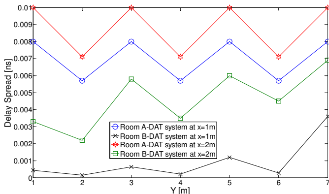
Fig.18: Delay spread of DAT imaging system in two different environments (rooms A and B) at x=1\text{m} and x=2\text{m} along y -axis.
