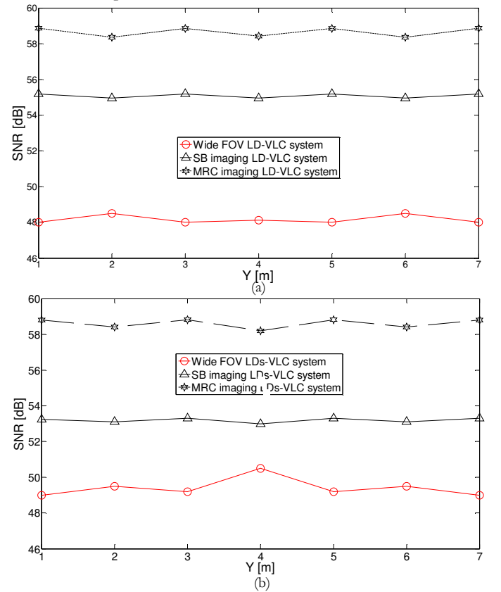
Fig.10: SNR of the two systems operating at 30 Mbps and using two combining schemes (SB and MRC for imaging receiver), (a) at x=1m and (b) at x=2m along the y -axis.
