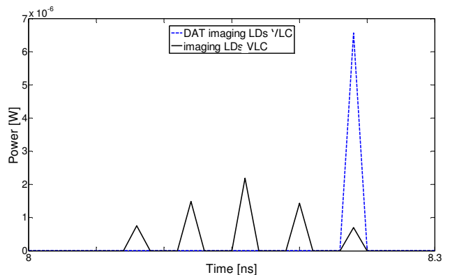
Fig.12: Impulse responses of the two systems at room centre (2m, 4m, 1m).
