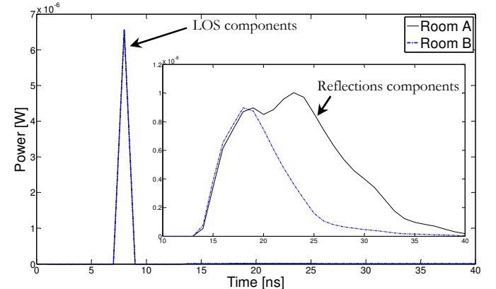
Fig.16: Impulse responses of DAT imaging system at room centre (2m, 4m, 1m) in two different environments (rooms A and B).
