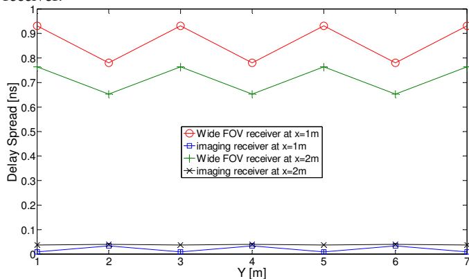
Fig.8: Delay spread of the wide FOV and the imaging LD-VLC systems in fourteen different locations when all the receivers move along the y-axis.
