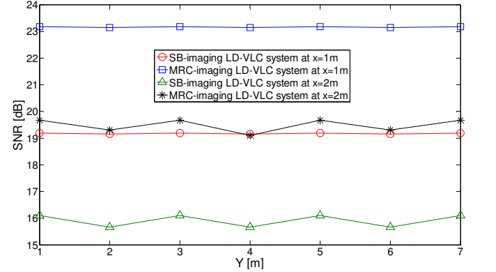
Fig.11: SNR of imaging LD-VLC system operating at 5 Gbps and using two combining schemes (SB and MRC), at x=1m and x=2m along the y -axis.
