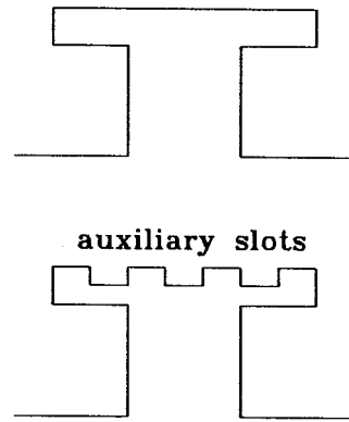
Fig. 7. Introduction of auxiliary slots.
