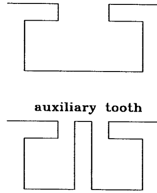
Fig. 6. Introduction of auxiliary teeth.
