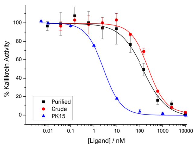
Figure 2. The inhibition of human plasma kallikrein by the mixture of stereoisomers 13 . ▲ PK15 LLL Ligand 8 ( IC_{50} 2.7 ± 0.10 nM) ■ Purified mixture of isomers 13 ( IC_{50} 144 ± 31 nM) ● Crude reaction mixture in the conversion of 12 to 13 . ( IC_{50} 238 ± 21 nM)
