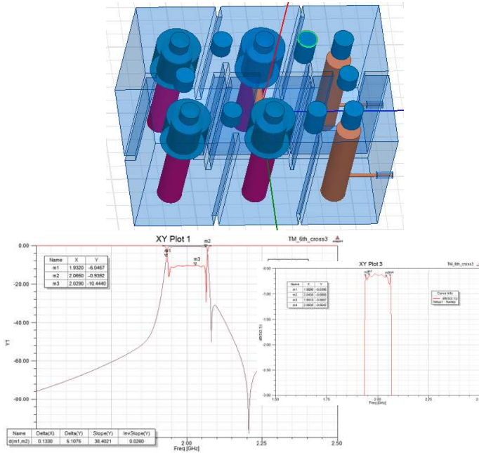
Fig. 1. EM model and response of the 6 th order mixed coaxial and TM mode dielectric filter
