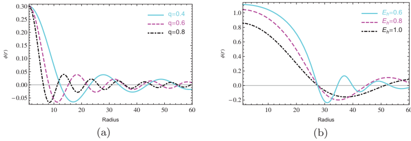
Fig. 2. The scalar field \phi(r) is plotted as a function of radius (a) for fixed \phi_h = 0.3 , E_h = 0.6 and different values of q , (b) for fixed q = 0.1 and different values of E_h .
