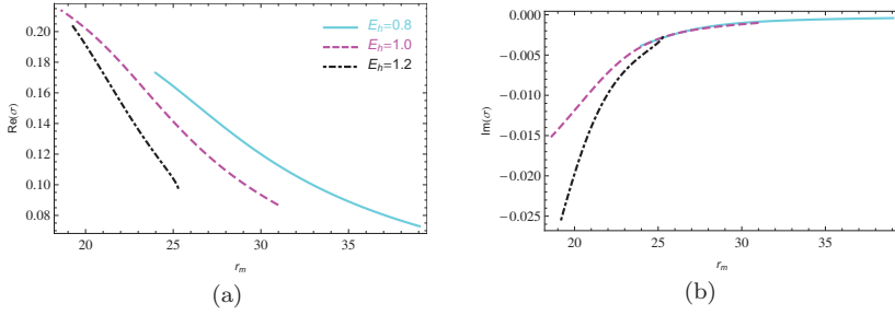
Fig. 3. The real (a) and imaginary part (b) of the perturbation frequency \sigma are plotted against the location of the mirror r_m with the scalar charge is fixed at q = 0.1 , \phi_h varying from 0.1 to 1.4 and different values of E_h .
