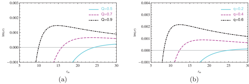
Fig. 1. The imaginary part of \sigma is plotted as a function of the location of the mirror r_m , (a) for fixed scalar charge q = 0.5 and different values of the black hole charge Q , (b) for fixed Q = 0.9 and different values of q .
