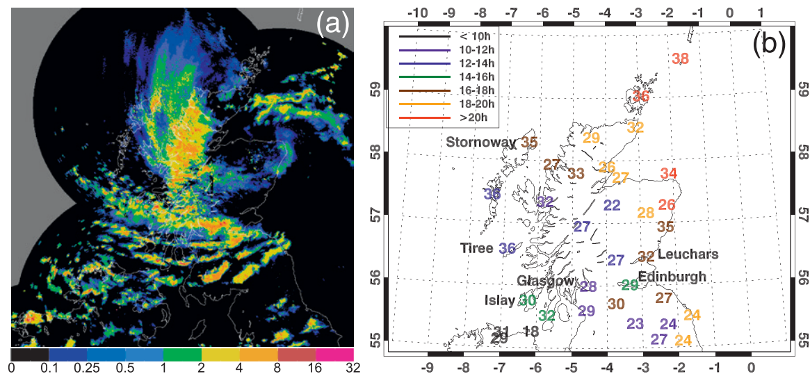
FIG. 4. (a) Radar-derived precipitation rate ( \text{mm h}^{-1} ) at 1800 UTC 8 Dec 2011 when the cyclone center had crossed to northeast Scotland and the banding to the south was most prominent. (b) Maximum 1-min gusts at surface stations over central Scotland during 8 Dec 2011, filtered using a 10-min median. Gust strength ( \text{m s}^{-1} ) is colored by the time of occurrence according to scale in the top-left corner of the panel.
