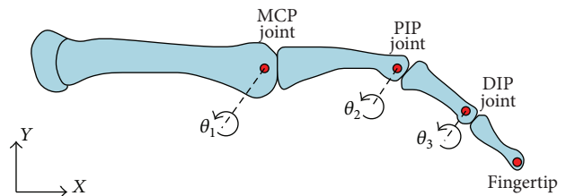
FIGURE 3: Planar skeletal model of the human finger.
