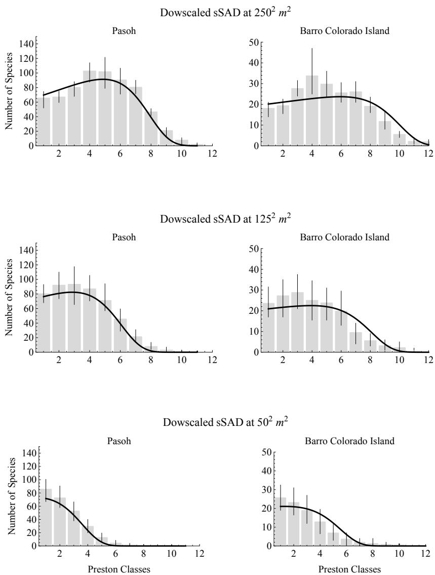
Figure 3: Species abundance distributions predicted by the theory at finer spatial scales. Solid curves are predictions of the spatial Species Abundance Distribution (sSAD) within sub-areas of the study region. The parameters are those used in Fig.(2) for BCI and Fig.S6 for Pasoh. Grey histograms represent empirical data. The area for which we downscaled the sSAD is indicated in the plot label. We divided the whole study region into equal non-overlapping square sub-areas, calculated the Preston classes of abundances as in Volkov et al. (2003) within each sub-area and finally averaged across sub-areas for each corresponding bin. Errors bars in each bin represent 95% confidence intervals as obtained from the empirical data.
