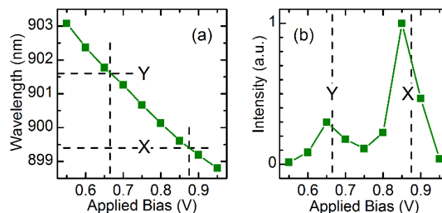
Figure 3. Single-dot line wavelength (a) and intensity (b) as a function of bias in the spectra collected from the cavity. Solid lines are guides for the eye. Horizontal dashed lines indicate the wavelengths of the cavity X- and Y-mode maxima; vertical dashed lines indicate the voltages at which the dot line is observed at these wavelengths.
