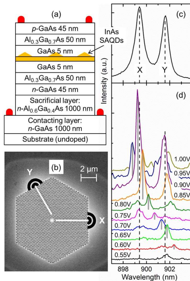
Figure 2. (a) Schematic diagram of the sample wafer. The contacts are shown by red semi-circles. (b) An electron microscope image of a typical photonic crystal membrane with an H1 cavity. X and Y denote W1 waveguides terminating by Bragg outcouplers. (c)-(d) Photoluminescence spectra from the cavity. (c) Spectra at high excitation power of 35 \mu\text{W} and bias of 1.1 V. X and Y denote X- and Y-dipole modes. (d) Series of spectra at low excitation power of 1 \mu\text{W} at various biases. Spectra are offset for clarity. A single-dot peak which crosses both cavities is highlighted by grey vertical bars. Vertical dashed lines indicate wavelengths of the cavity mode maxima.
