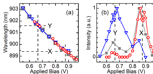
Figure 4. Single-dot line wavelength (a) and intensity (b) as a function of bias in the spectra collected from the cavity, X and Y outcouplers (grey squares, red circles and blue triangles, respectively). Line intensities are normalized. The meaning of the dashed lines is the same as in Fig. 3.
