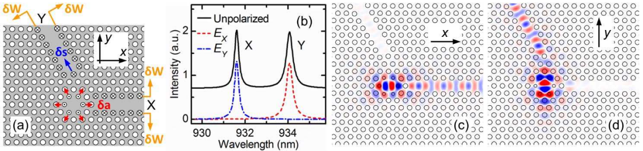
Figure 1. (a) Schematic diagram of the photonic crystal design, showing the H1 cavity and two W1 waveguides, X and Y. For device optimisation, holes adjacent to the waveguides and to the cavity (denoted by crosses and dots, respectively) are displaced, as indicated by arrows; in addition, the radius of the ring of holes adjacent to the cavity centre is reduced. (b)-(d) Results of modelling for waveguide-coupled non-degenerate cavity modes. (b) Cavity mode spectra for non-polarised, x - and y -polarised dipole sources (solid black, dashed red and dash-dotted blue, respectively). The non-polarised spectrum is offset for clarity. X and Y denote X- and Y-dipole modes, see discussion in the text. (c) Normalised H_z profile for the X-dipole mode. A linear red-white-blue colour scale represents field strength in the range from -92\% to 92\% , with positive and negative values shown by red and blue, respectively. Magnitudes below -92\% and above 92\% are shown by saturated colours. (d) The same as (c) for the Y-dipole mode.
