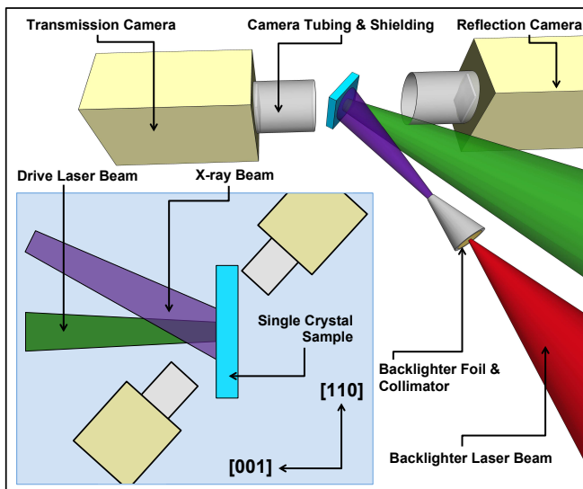
FIG. 1. Schematic diagram of the experimental setup. Inset: Top-down view of the experiment highlighting orientation relative to crystal axes.
