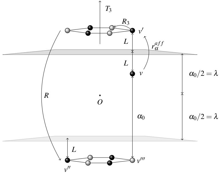
Figure 4: Translations and twist translations can be generated by affine reflection planes perpendicular to 3- and 5-fold rotational symmetry axes of icosahedral symmetry. Assume that there is an affine reflection plane at a distance \lambda = \frac{\alpha_0}{2} from the origin (but no corresponding parallel plane through the origin). Any vector v at a distance L below the affine reflection plane can be reflected to a vector v' at a position L above it. The rotational part of the group ( R_3 and R_5 ) then generates a triangle around the 3-fold axis (black points), or a pentagon around a 5-fold axis, and the full group H_3 generates a hexagon (additional white points), or a decagon, respectively. By using a rotation R in the group, these can be rotated into a parallel plane at a distance 2\lambda + L from the affine reflection plane and at a distance \lambda + L from the origin (note that v'' is part of this plane). As the generators R_3 and R_5 allow to rotate any point in the hexagon and decagon into any other, one of these rotations can be used to align the reflected and rotated v (the point v'' ) with the initial v (yielding a point v''' ) such that v and v''' differ by a translation of length 2\lambda = \alpha_0 along T_3 (resp. T_5 ). The other 5 (9 respectively) rotations also generate twist translations.
